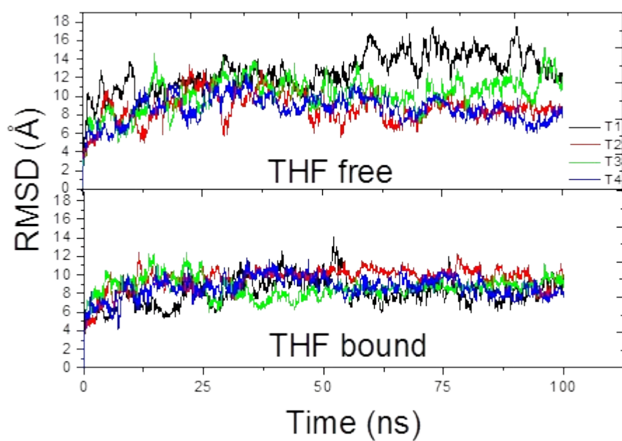
Figure S1. C5' RMSD for THF free and bound systems.
