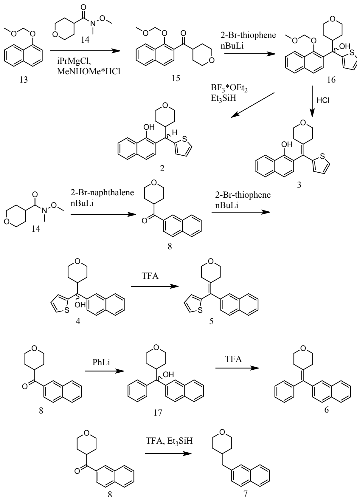
Fig. S1: Synthesis of compounds 2-8. see synthetic methods section for details
