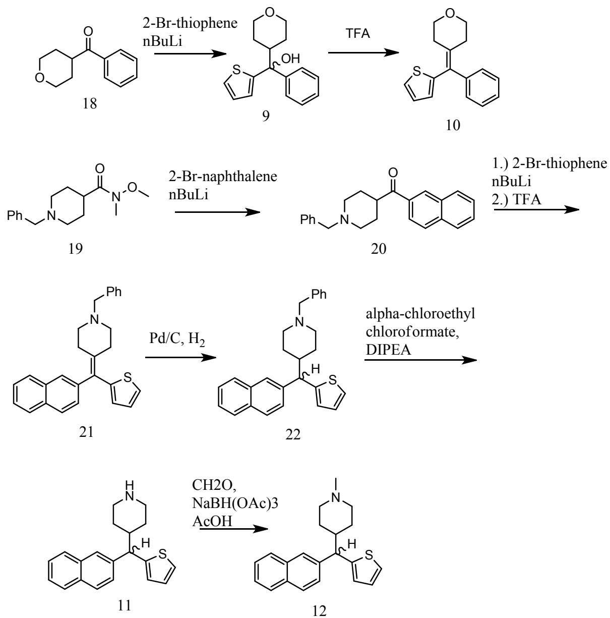
Fig. S2: Synthesis of compounds 9-12. see synthetic methods section for details
