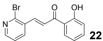
(E) -3-(2-Bromopyridin-3-yl)-1-(2-hydroxyphenyl)-2-propen-1-one
