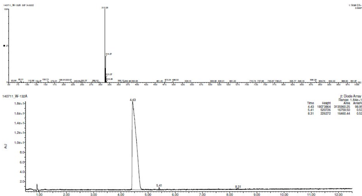
Compound 17
