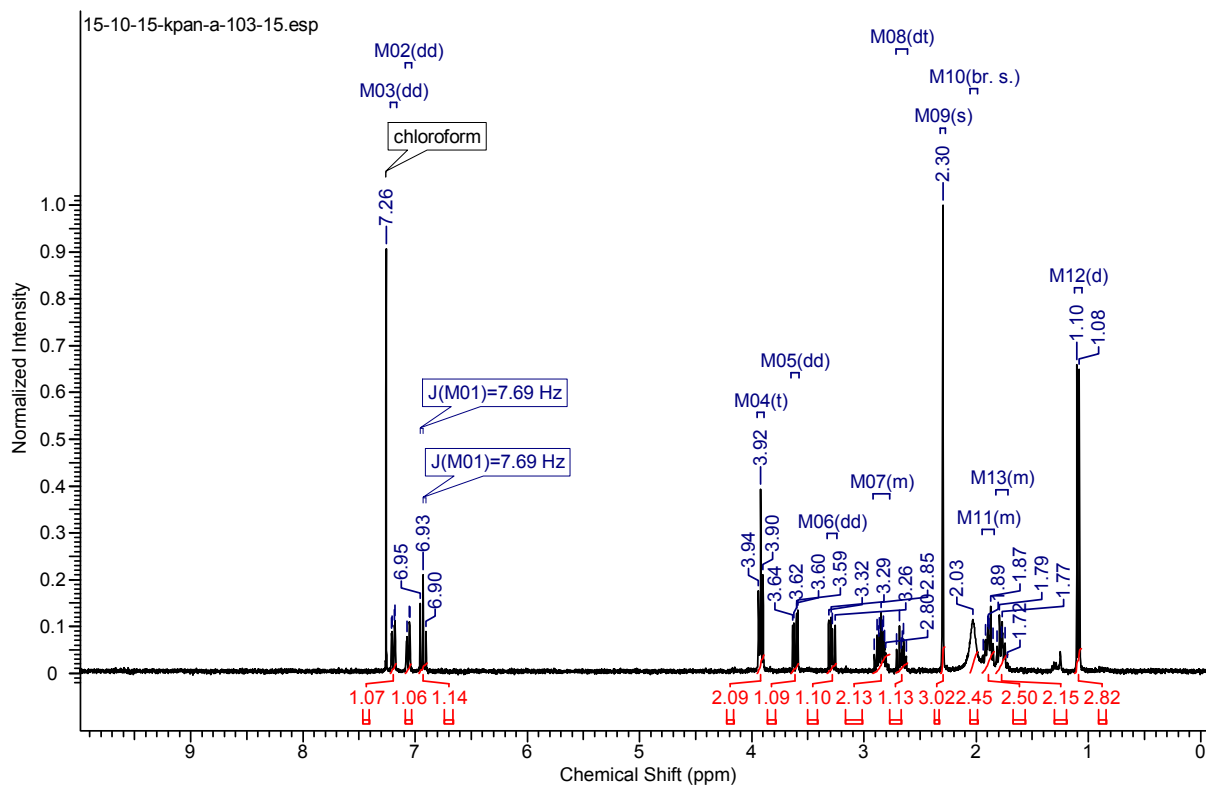
Compound 17
