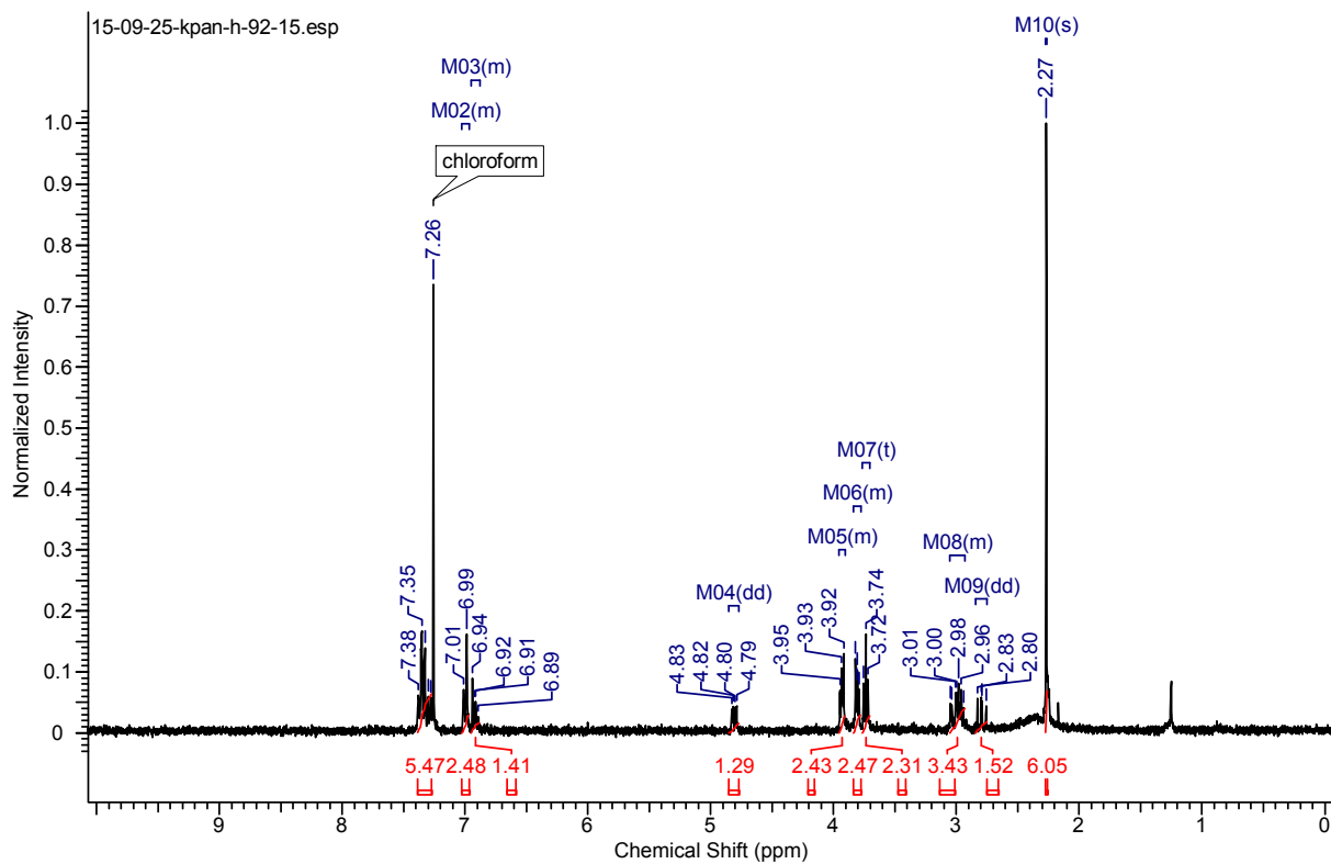
Compound 24
