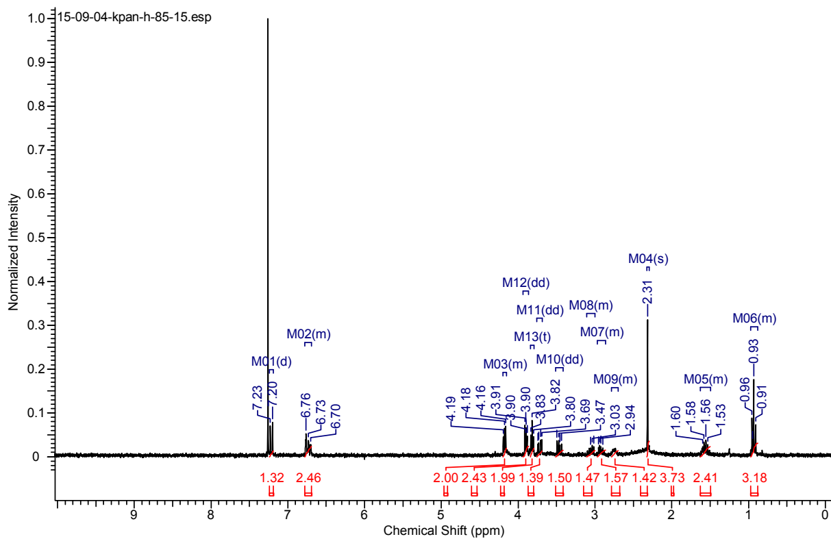
Compound 26
