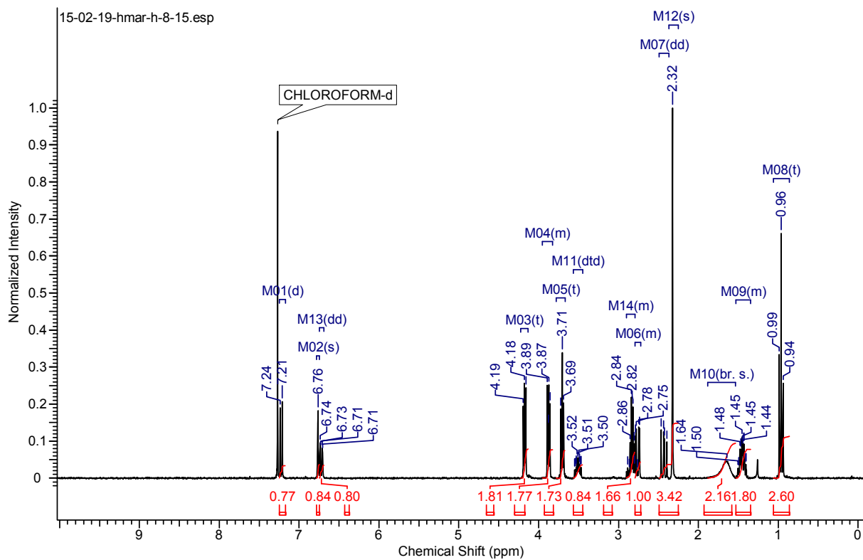
Compound 25
