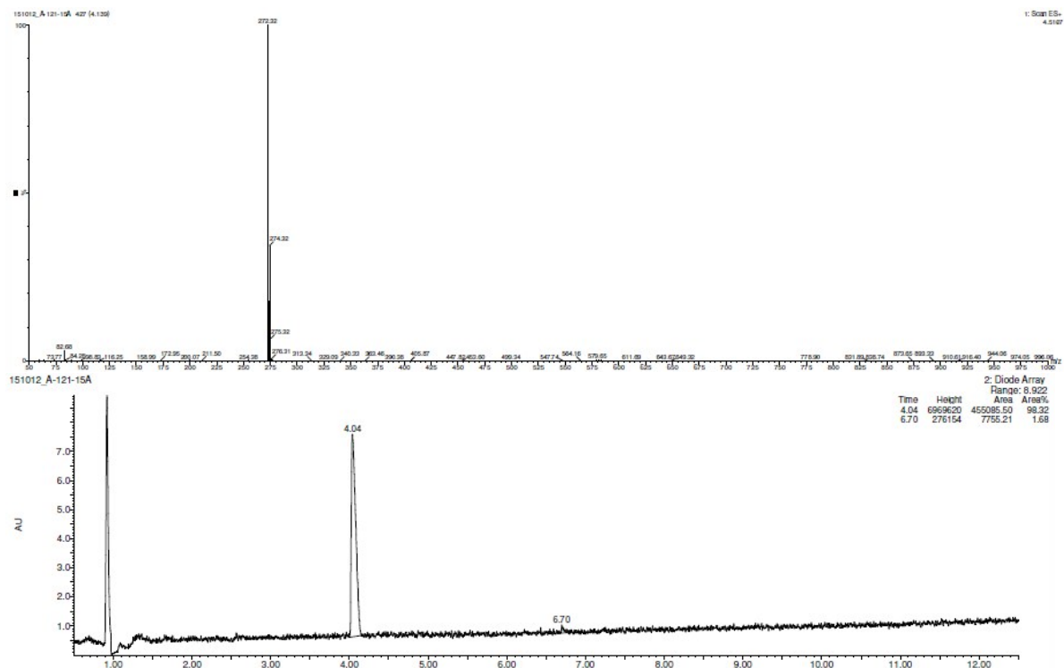
Compound 16
