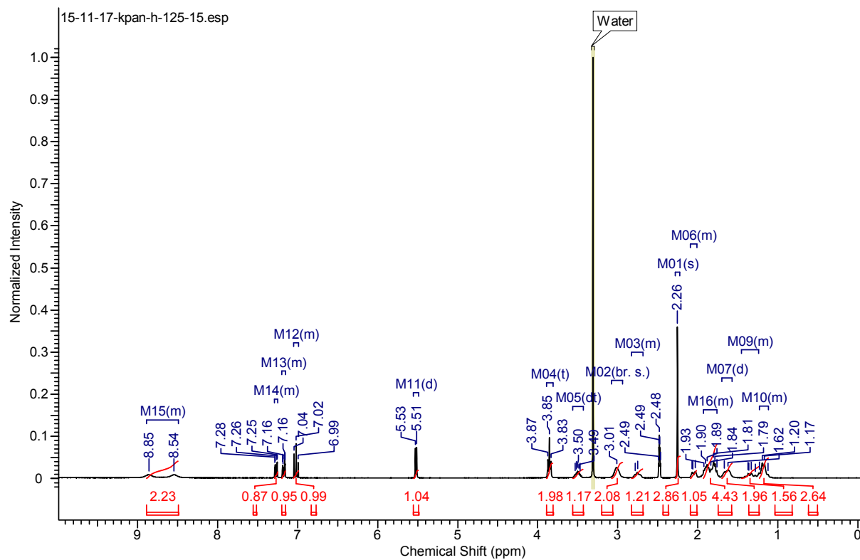
Compound 18
