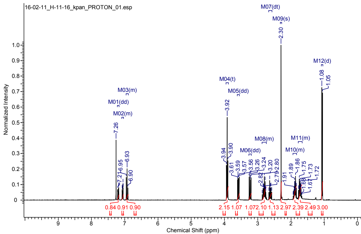
Compound 16
