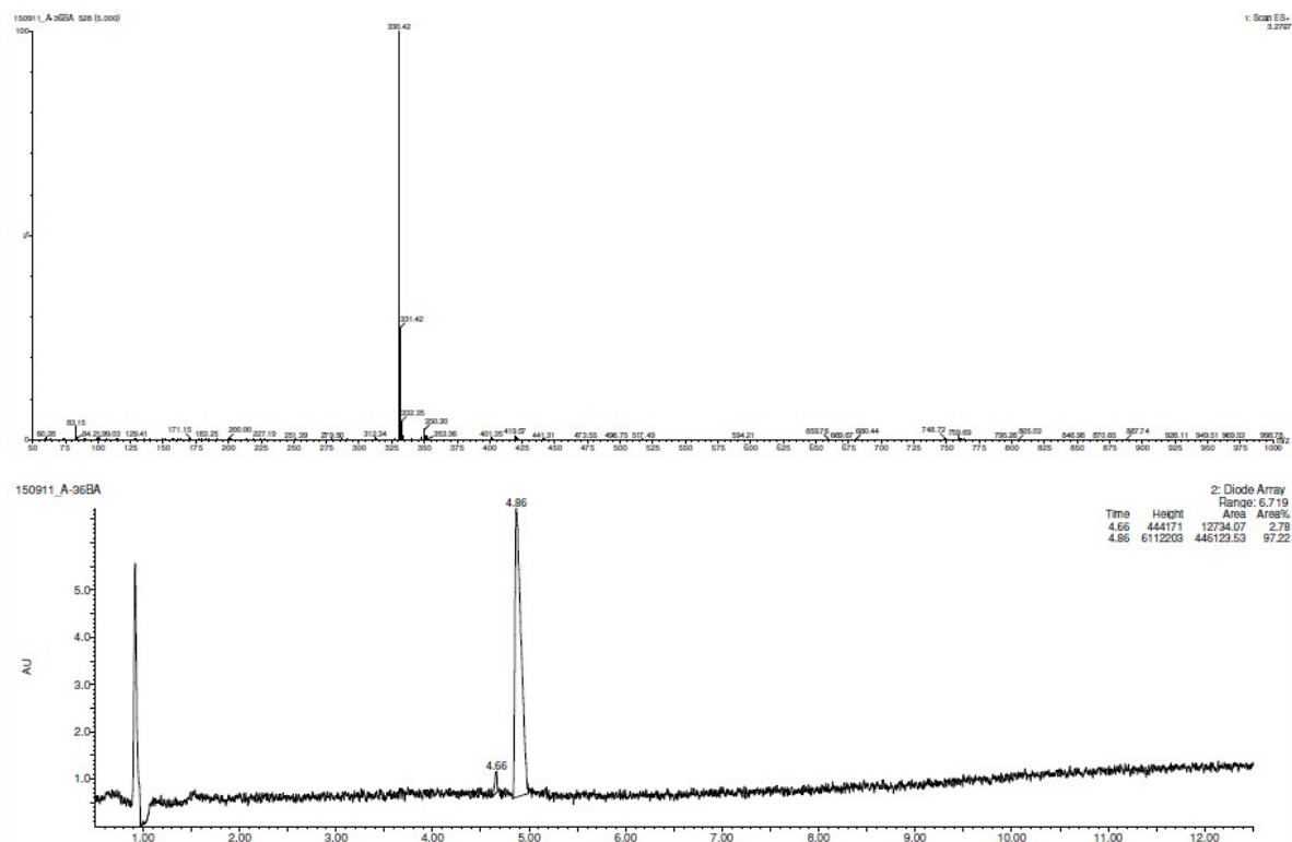
Compound 23
