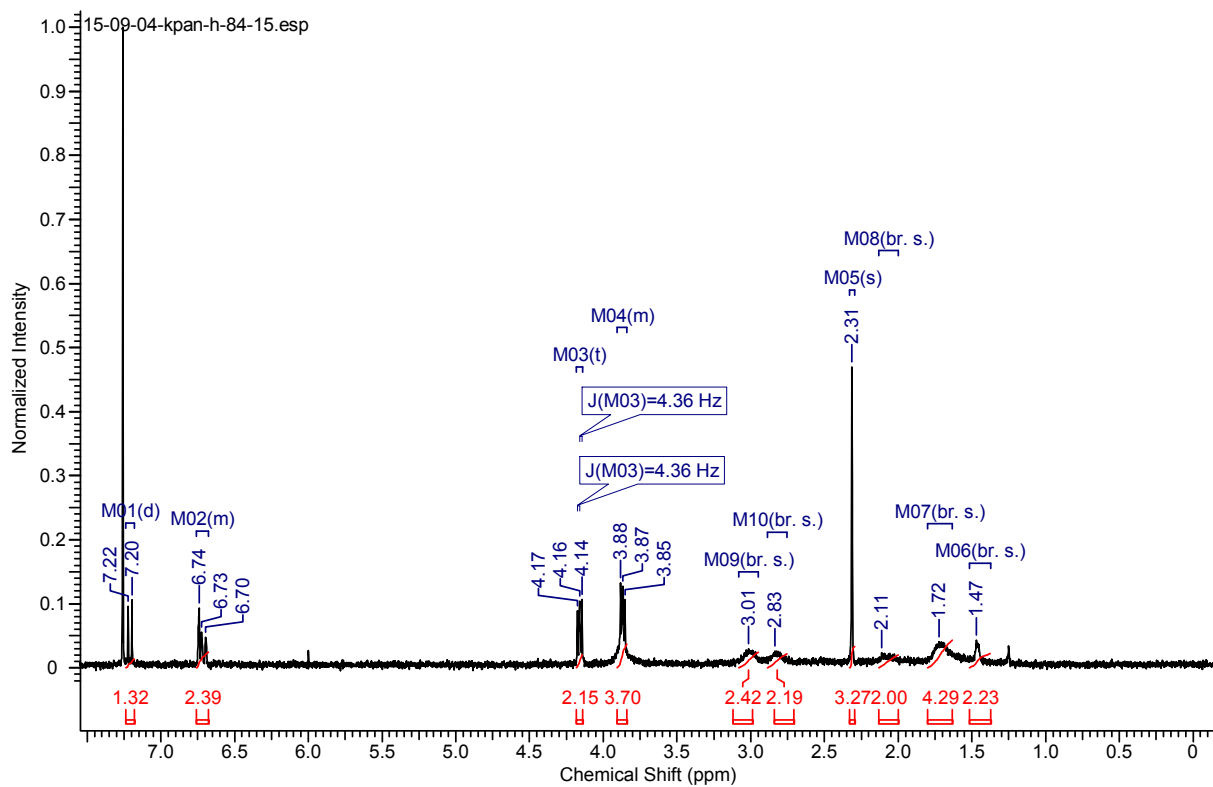
Compound 27
