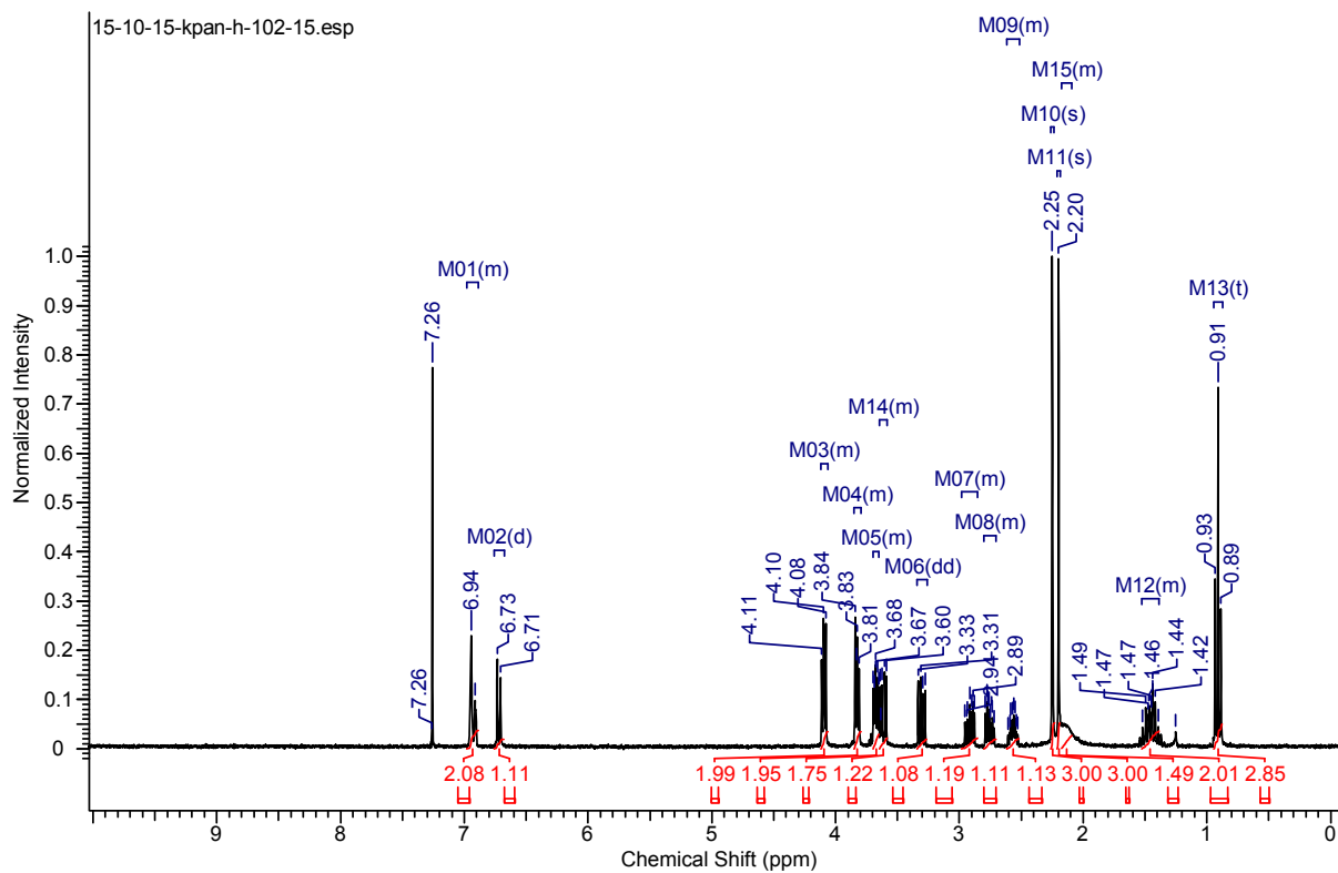
Compound 23
