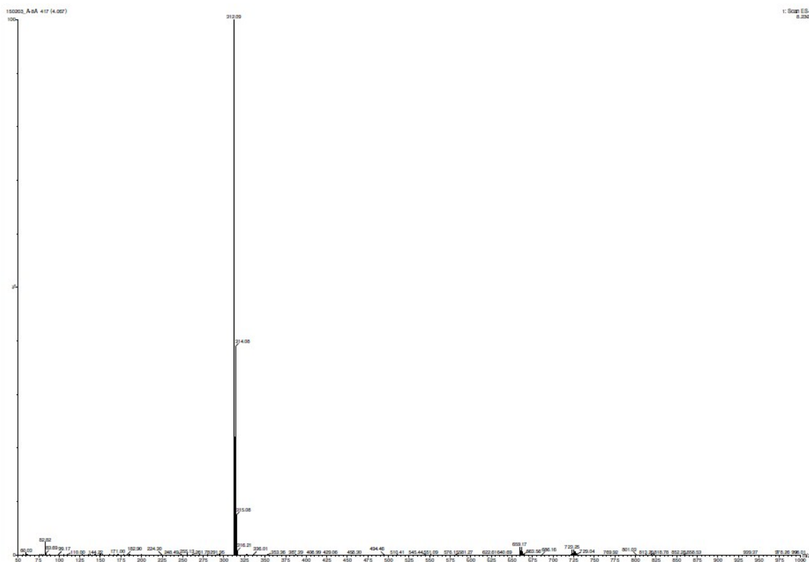
Compound 18
