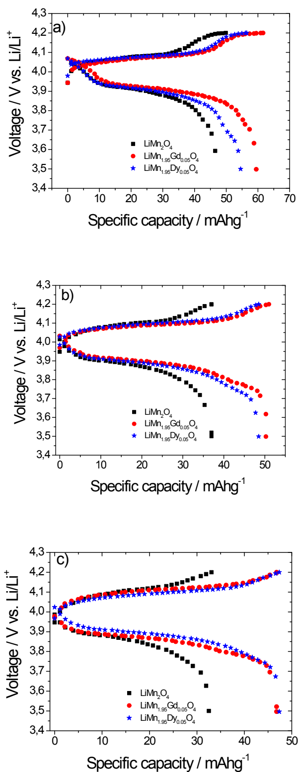
Fig. S1- Charge-discharge profile of \text{LiMn}_2\text{O}_4 , \text{LiMn}_{1.95}\text{Gd}_{0.05}\text{O}_4 and \text{LiMn}_{1.95}\text{Dy}_{0.05}\text{O}_4 based electrodes for the 5 th (a), 25 th (b) and 45 th (c) cycles at C/2.
