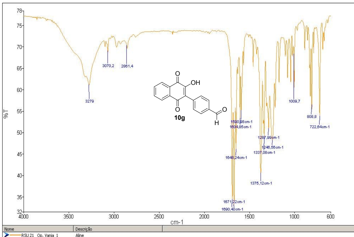
Figure S29 - Infrared spectrum of 4-(3-hydroxy-1,4-dioxo-1,4-dihydronaphthalen-2-yl)benzaldehyde ( 10g )
