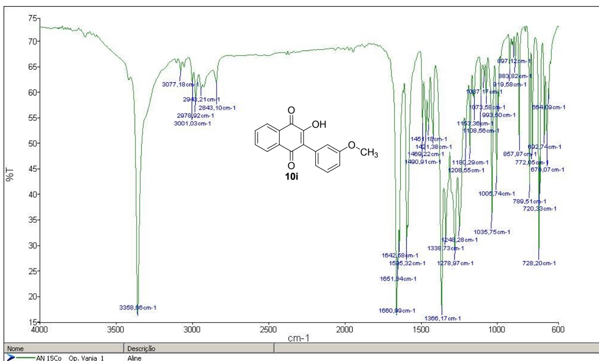
Figure S35 - Infrared spectrum of 2-hydroxy-3-(3-methoxyphenyl)naphthalene-1,4-dione (10i)
