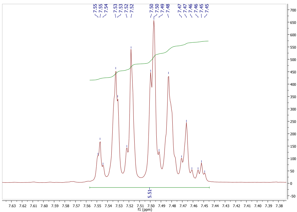
Figure S12 ^1\text{H} NMR Spectra of 2-hydroxy-3-phenylnaphthalene-1,4-dione ( 10a )
