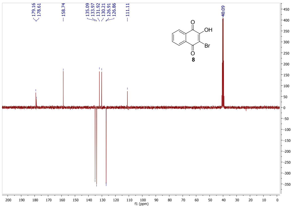
Figure S9 - ^{13}\text{C} NMR Spectra of 2-bromo-3-hydroxynaphthalene-1,4-dione ( 8 )
