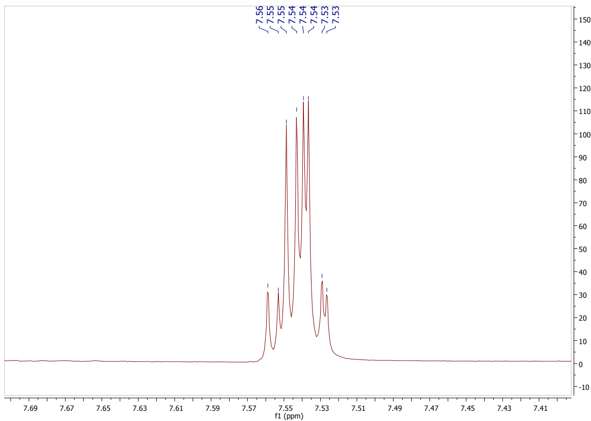
Figure S24 - ^1\text{H} NMR Spectra of 2-hydroxy-3-(thiophen-3-yl)naphthalene-1,4-dione ( 10e )
