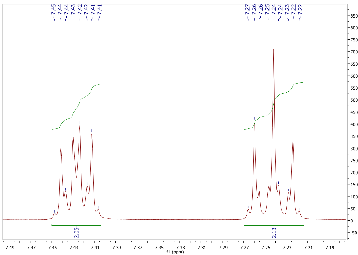
Figure S15 - ^1\text{H} NMR Spectra of 2-(4-fluorophenyl)-3-phenylnaphthalene-1,4-dione ( 10b )
