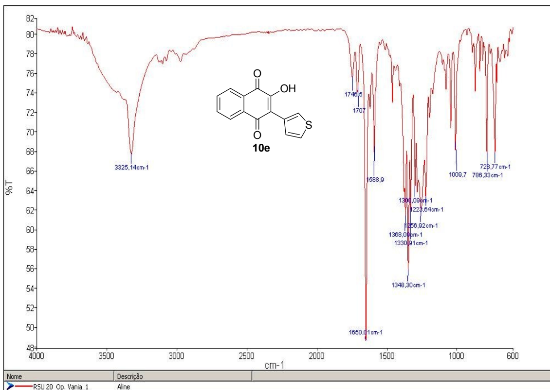
Figure S23 - Infrared spectrum of 2-hydroxy-3-(thiophen-3-yl)naphthalene-1,4-dione ( 10e )
