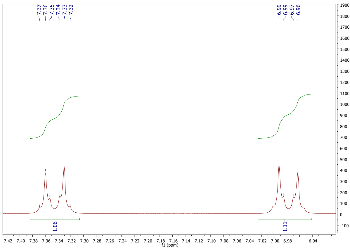
Figure S33 - ^1\text{H} NMR Spectra of 2-hydroxy-3-(4-methoxyphenyl)naphthalene-1,4-dione ( 10h )
