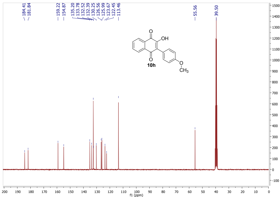
Figure S34 - ^1\text{H} NMR Spectra of 2-hydroxy-3-(4-methoxyphenyl)naphthalene-1,4-dione (10h)
