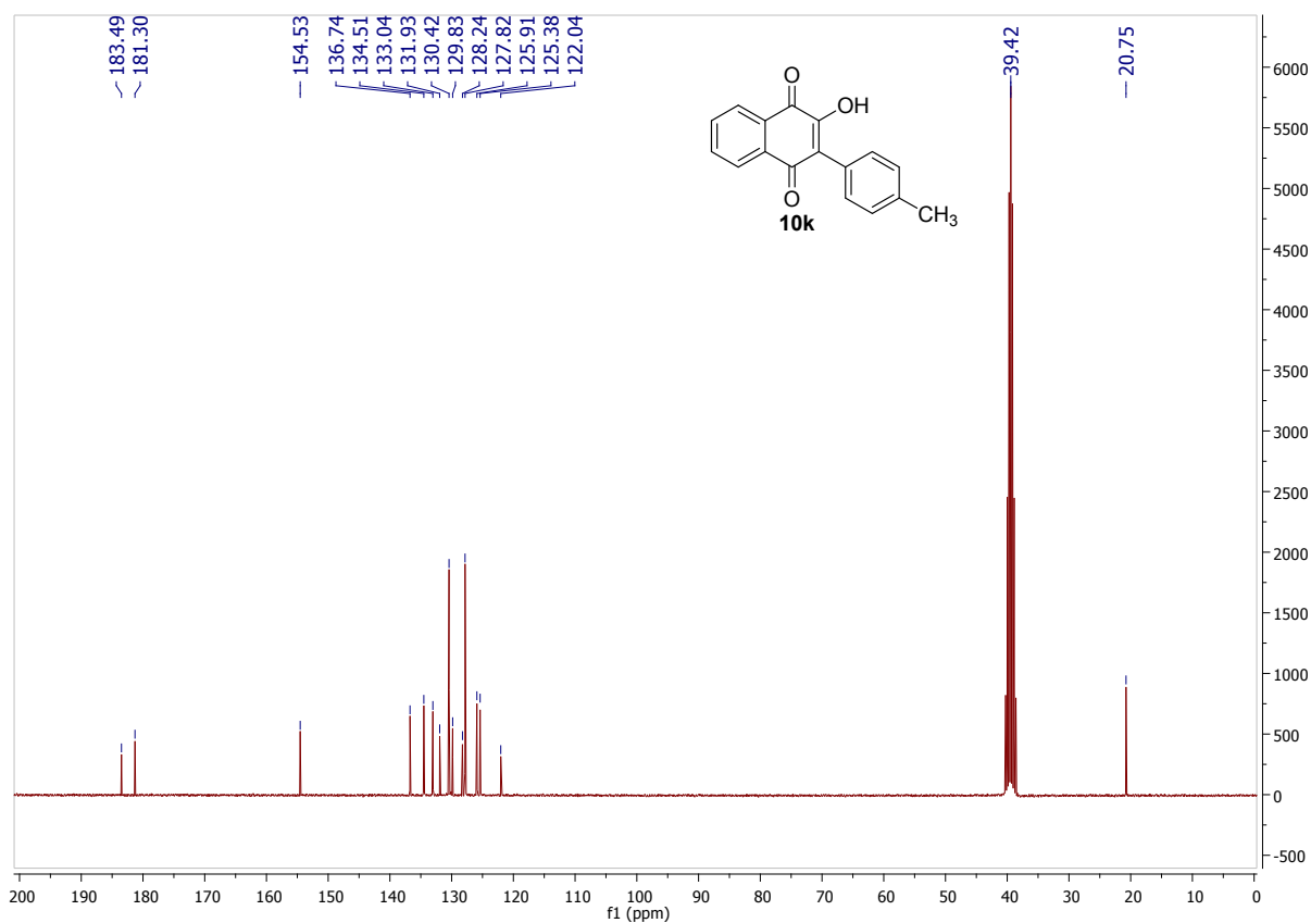
Figure S43 - 13 C NMR Spectra of 2-Hydroxy-3-( p -tolyl)naphthalene-1,4-dione ( 10k )
