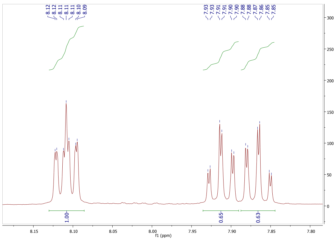
Figure S5 - ^1\text{H} NMR Spectra of 2-amino-3-iodonaphthalene-1,4-dione ( 7 )
