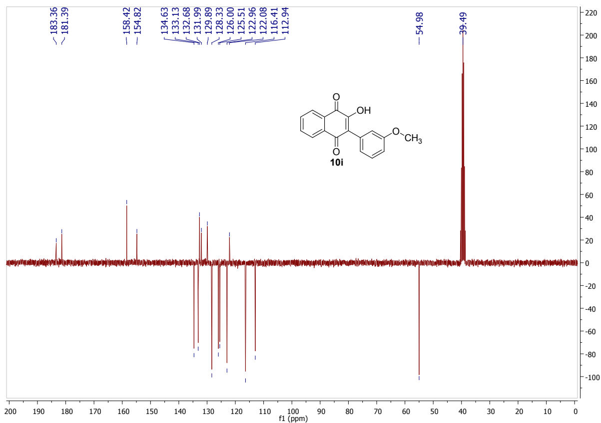
Figure S37 - ^{13}\text{C} NMR Spectra of 2-hydroxy-3-(3-methoxyphenyl)naphthalene-1,4-dione ( 10i )
