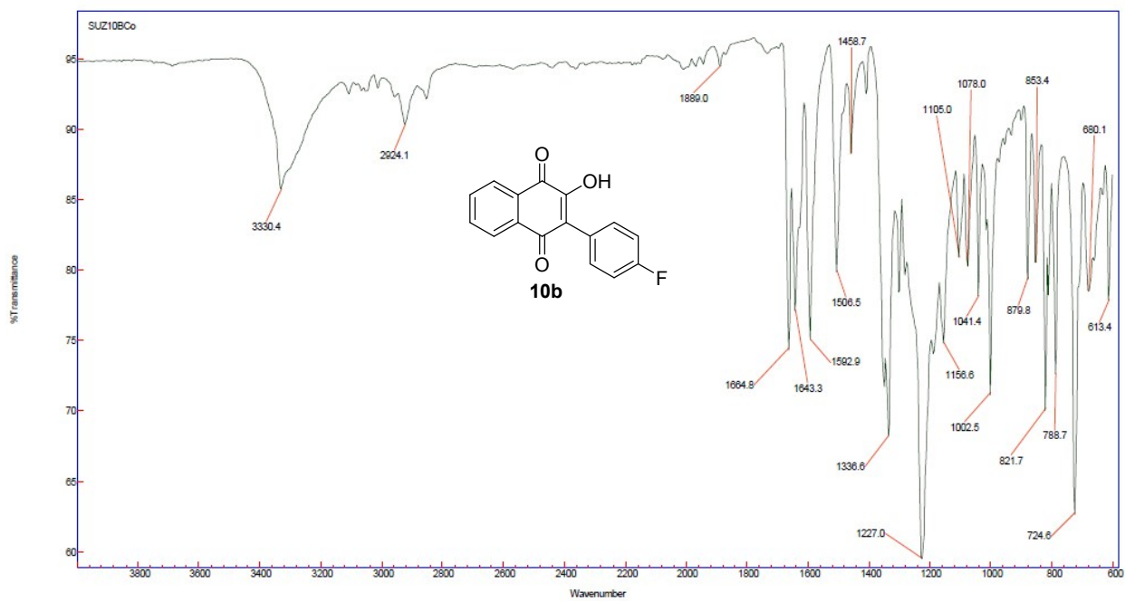
Figure S14 Infrared spectrum of 2-(4-fluorophenyl)-3-phenylnaphthalene-1,4-dione (10b)
