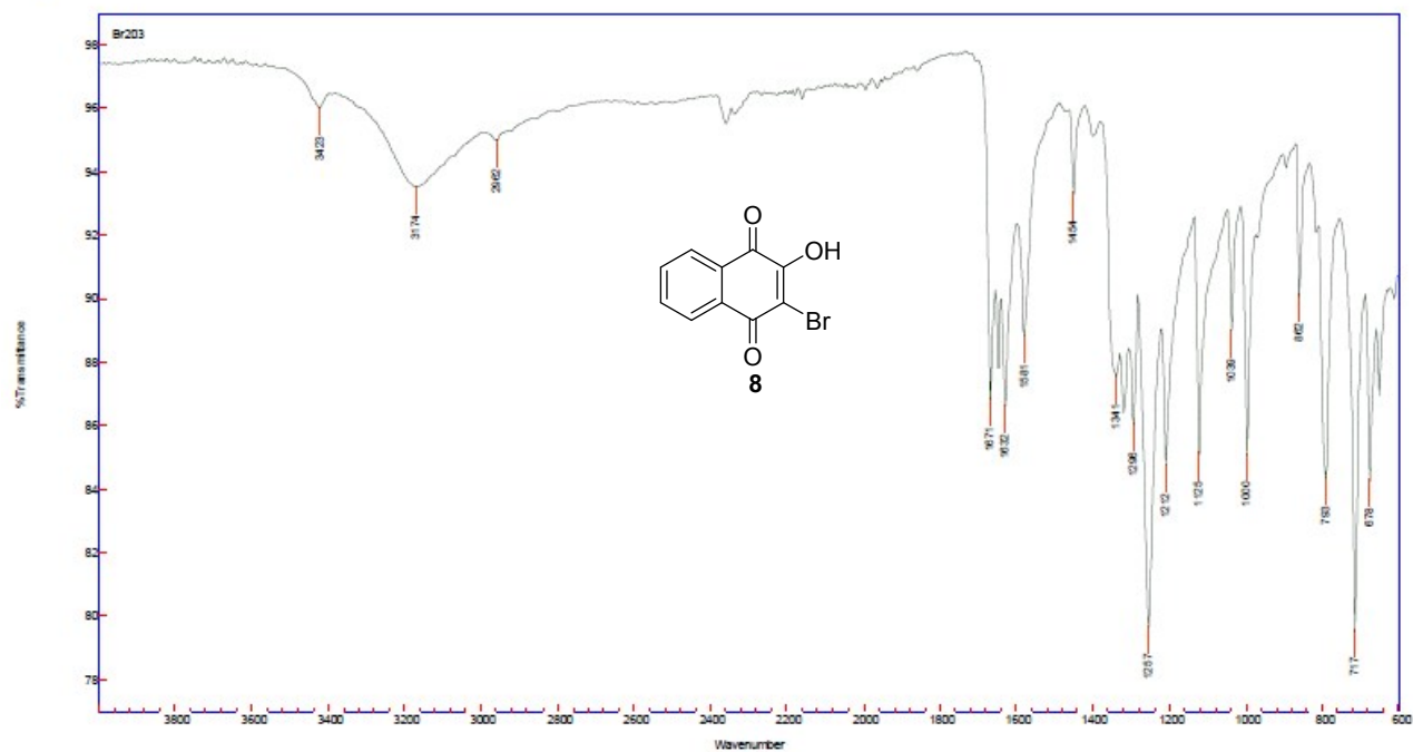
Figure S7 - Infrared spectrum of 2-bromo-3-hydroxynaphthalene-1,4-dione (8)
