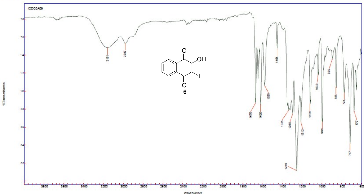
Figure S1 - Infrared spectrum of 2-hydroxy-3-iodonaphthalene-1,4-dione (6)
