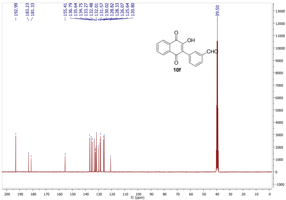
Figure S28 13 C NMR Spectra of 3-(3-Hydroxy-1,4-dioxo-1,4-dihydronaphthalen-2-yl)benzaldehyde ( 10f )
