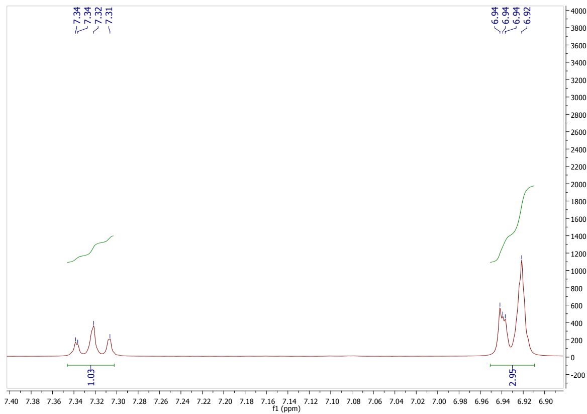
Figure S36 - ^1\text{H} NMR Spectra of 2-hydroxy-3-(3-methoxyphenyl)naphthalene-1,4-dione ( 10i )
