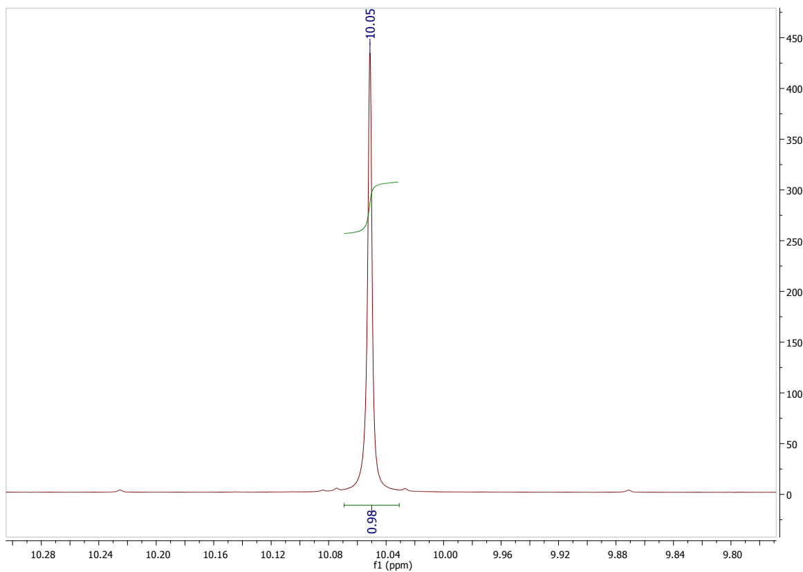
Figure S30 - ^1\text{H} NMR Spectra of 4-(3-hydroxy-1,4-dioxo-1,4-dihydronaphthalen-2-yl)benzaldehyde ( 10g )
