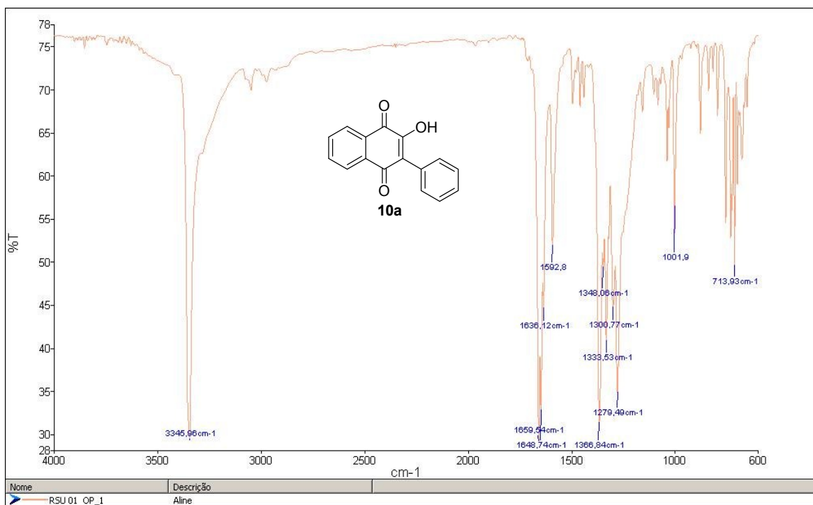
Figure S10 - Infrared Spectrum of 2-hydroxi-3-phenylnaphthalene-1,4-dione ( 10a )
