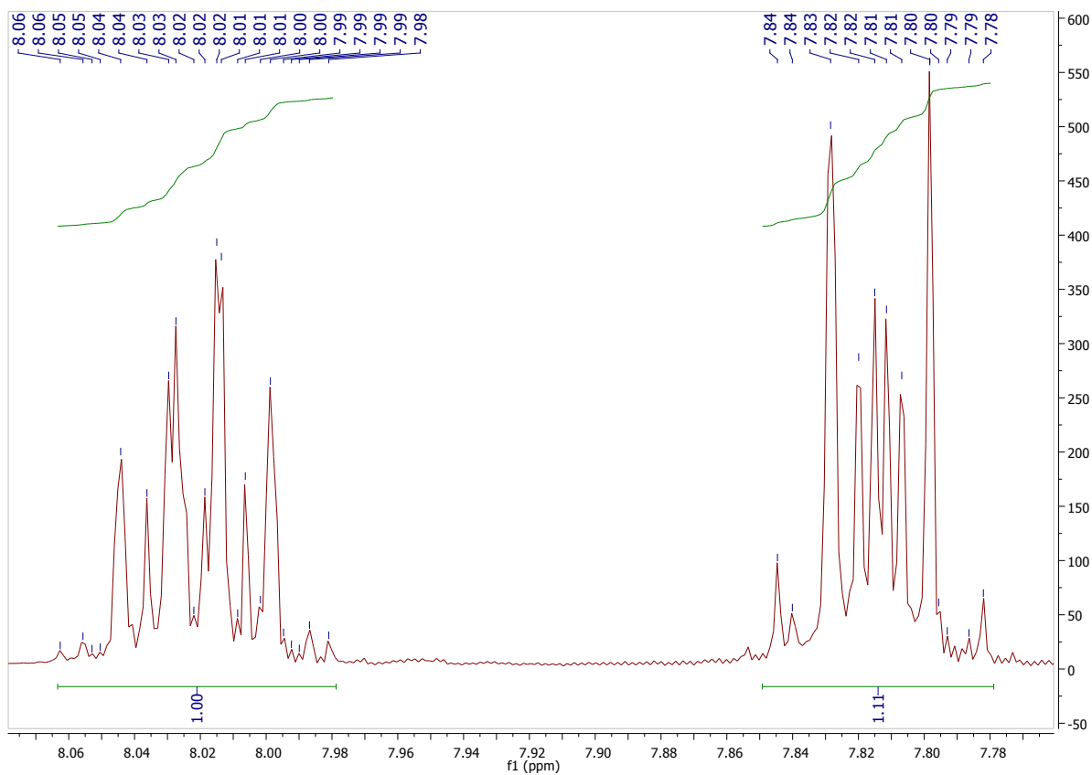
Figure S2 - ^1\text{H} NMR Spectra of 2-hydroxy-3-iodonaphthalene-1,4-dione ( 6 )
