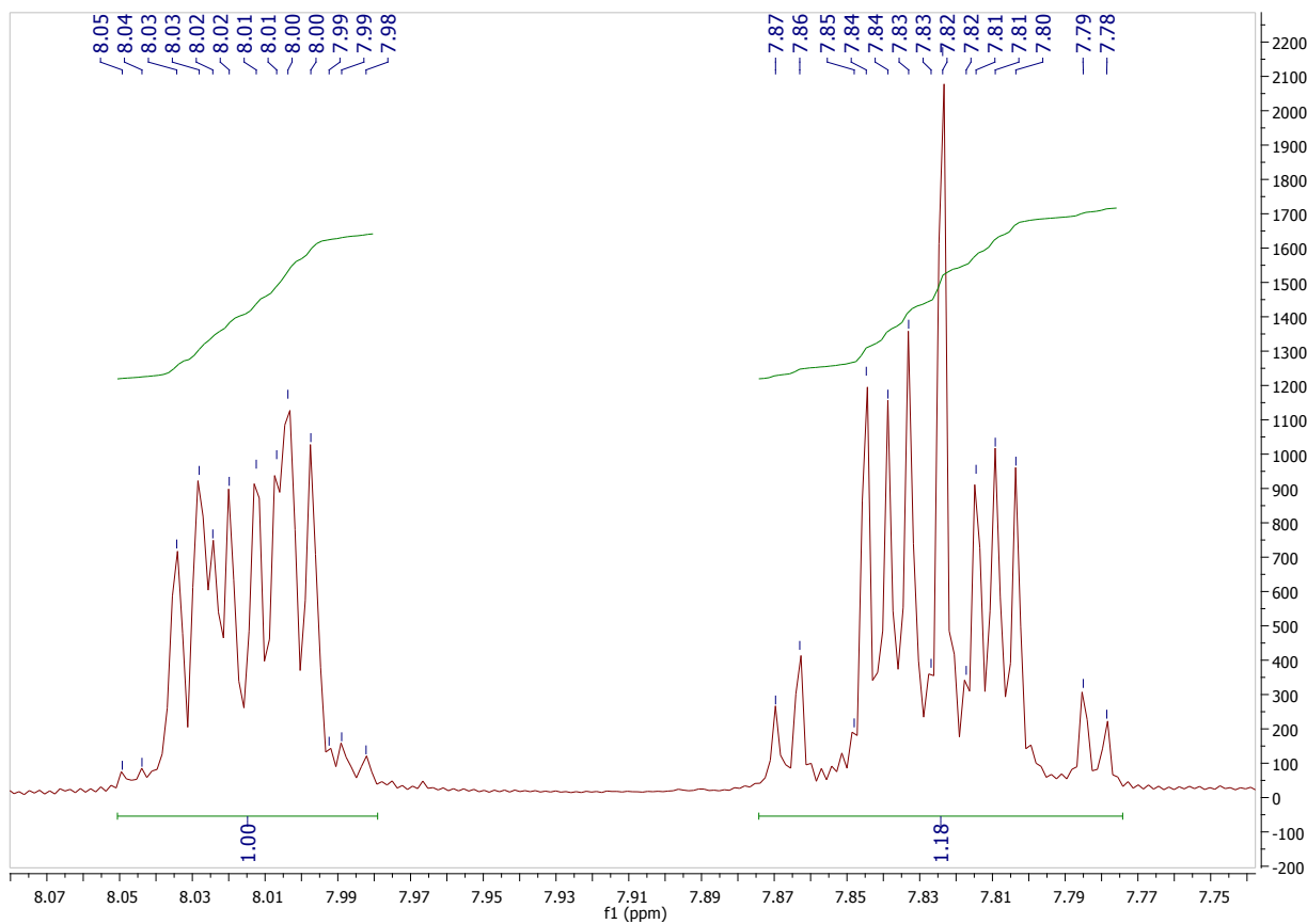
Figure S8 - ^1\text{H} NMR Spectra of 2-bromo-3-hydroxynaphthalene-1,4-dione ( 8 )
