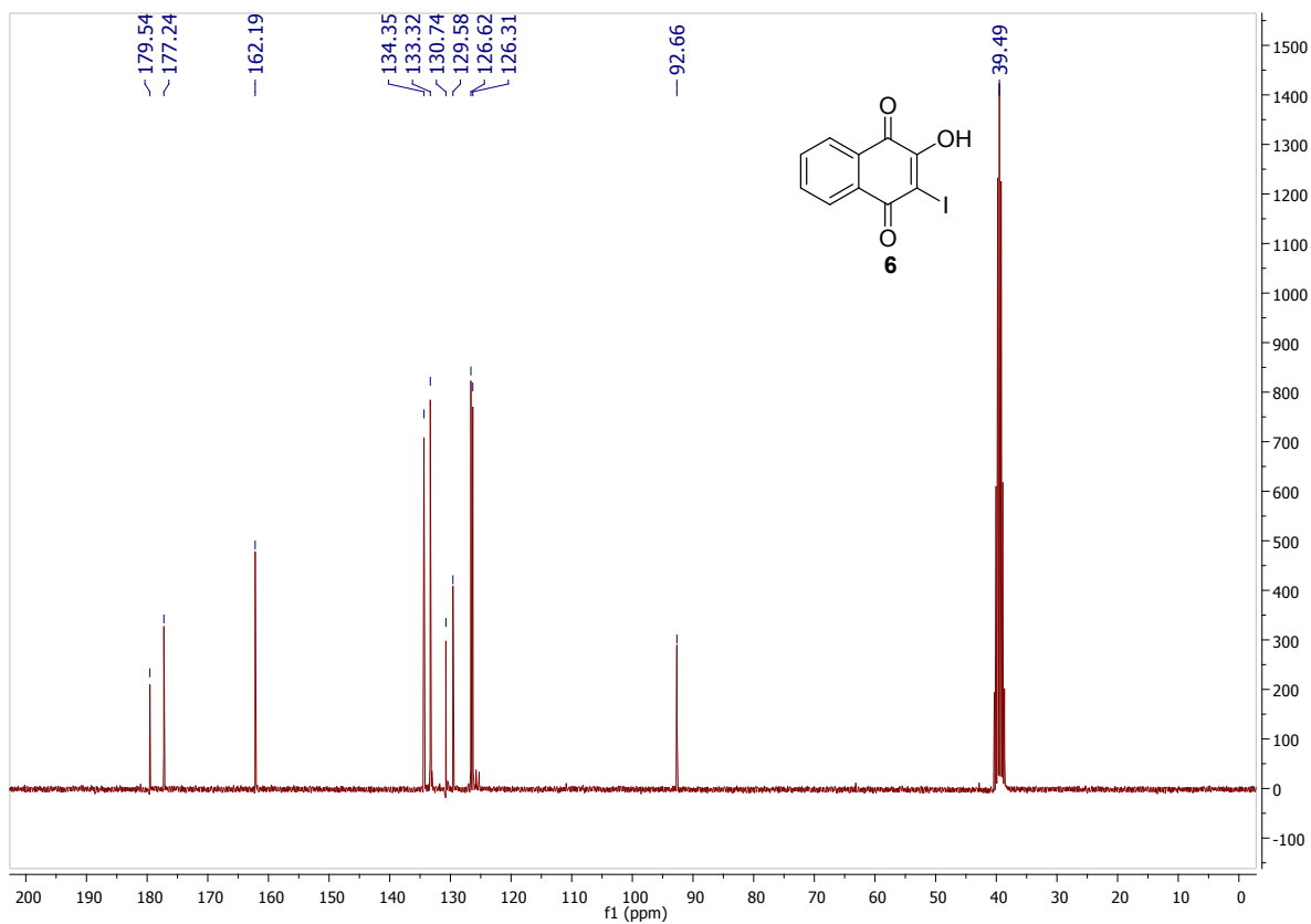
Figure S3 - ^{13}\text{C} NMR Spectra of 2-hydroxy-3-iodonaphthalene-1,4-dione (6)
