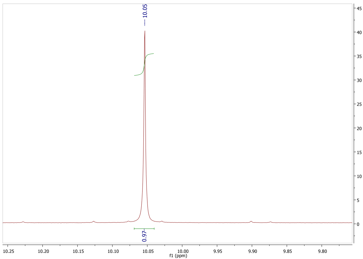
Figure S27 - ^1\text{H} NMR Spectra of of 3-(3-Hydroxy-1,4-dioxo-1,4-dihydronaphthalen-2-yl)benzaldehyde (10f)
