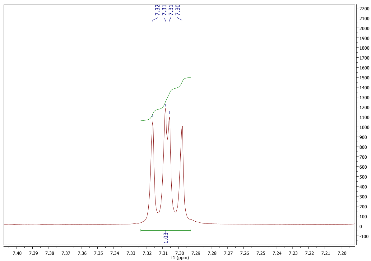
Figure S21 - 1 H NMR Spectra of 2-hydroxy-3-(thiophen-2-yl)naphthalene-1,4-dione ( 10d )
