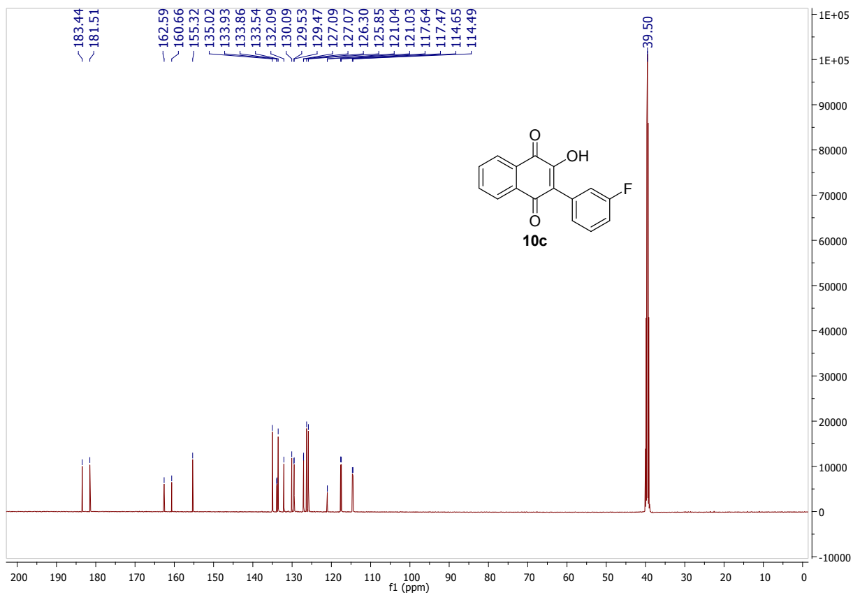
Figure S19 - ^{13}\text{C} NMR Spectra of 2-(3-fluorophenyl)-3-phenylnaphthalene-1,4-dione ( 10c )
