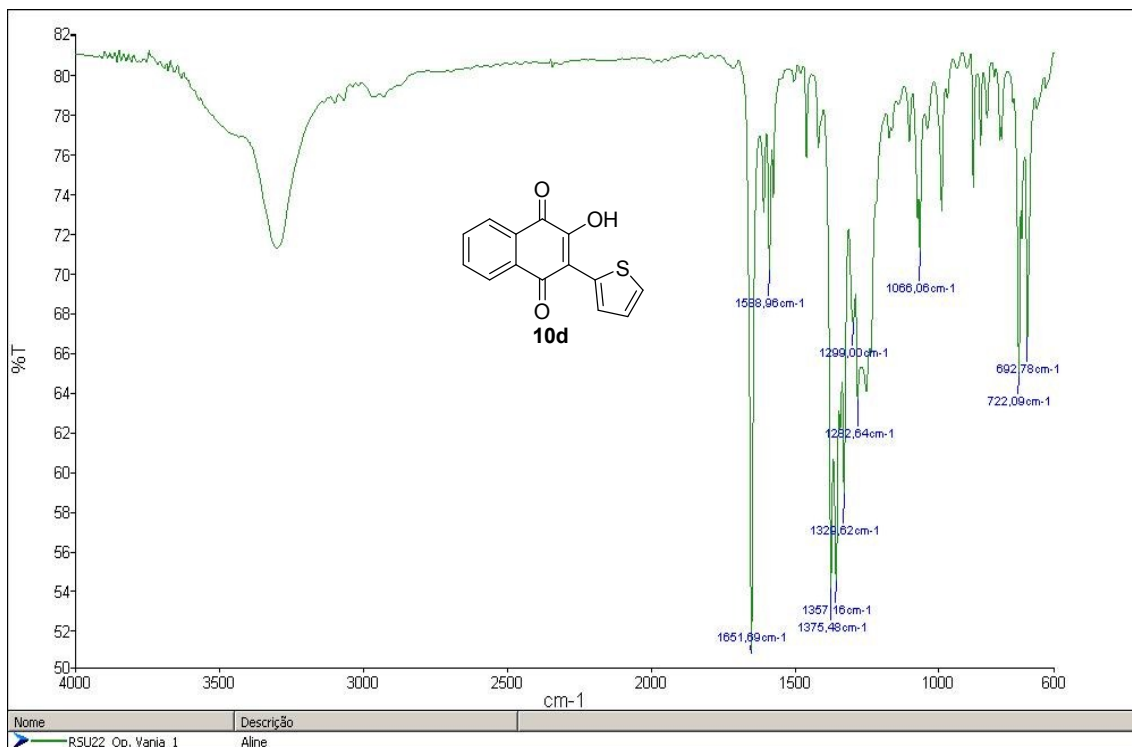
Figure S20 - Infrared spectrum of 2-hydroxy-3-(thiophen-2-yl)naphthalene-1,4-dione (10d)
