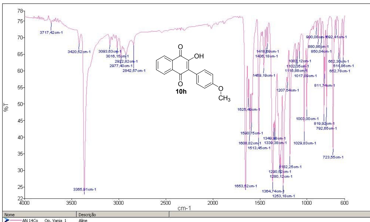
Figure S32 Infrared spectrum of 2-hydroxy-3-(4-methoxyphenyl)naphthalene-1,4-dione (10h)
