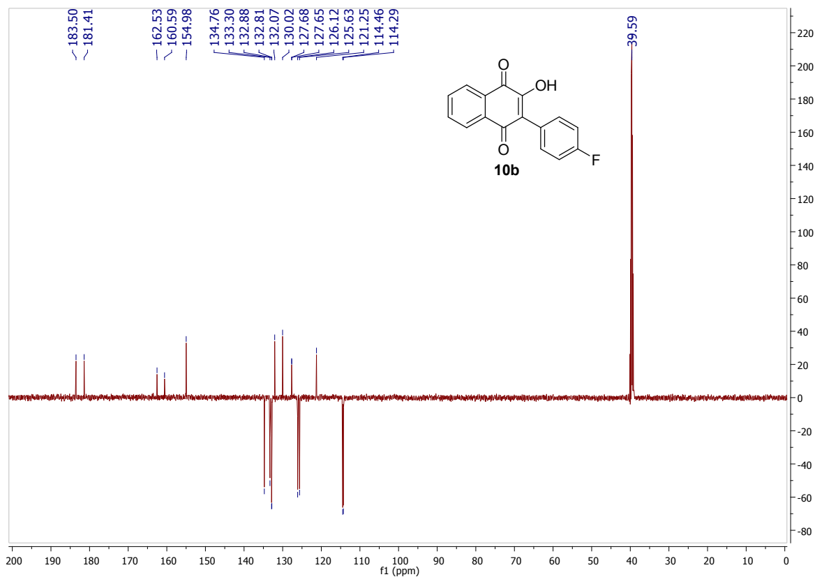
Figure S16 - 13 C NMR Spectra of 2-(4-fluorophenyl)-3-phenylnaphthalene-1,4-dione ( 10b )
