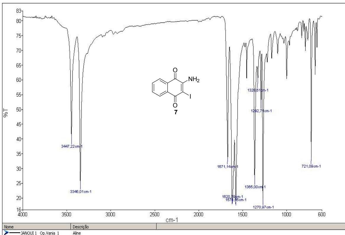
Figure S4 - Infrared spectrum of 2-amino-3-iodonaphthalene-1,4-dione (7)
