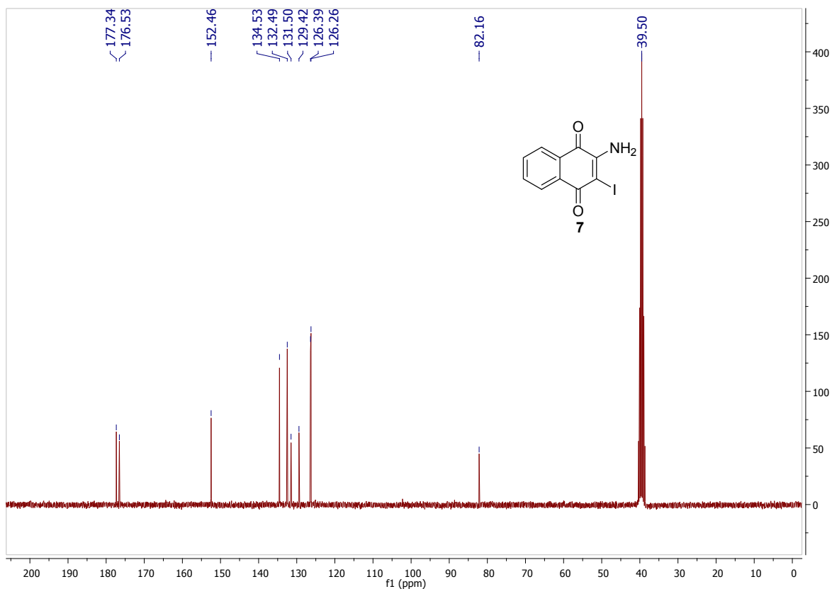
Figure S6 - ^{13}\text{C} NMR Spectra of 2-amino-3-iodonaphthalene-1,4-dione (7)
