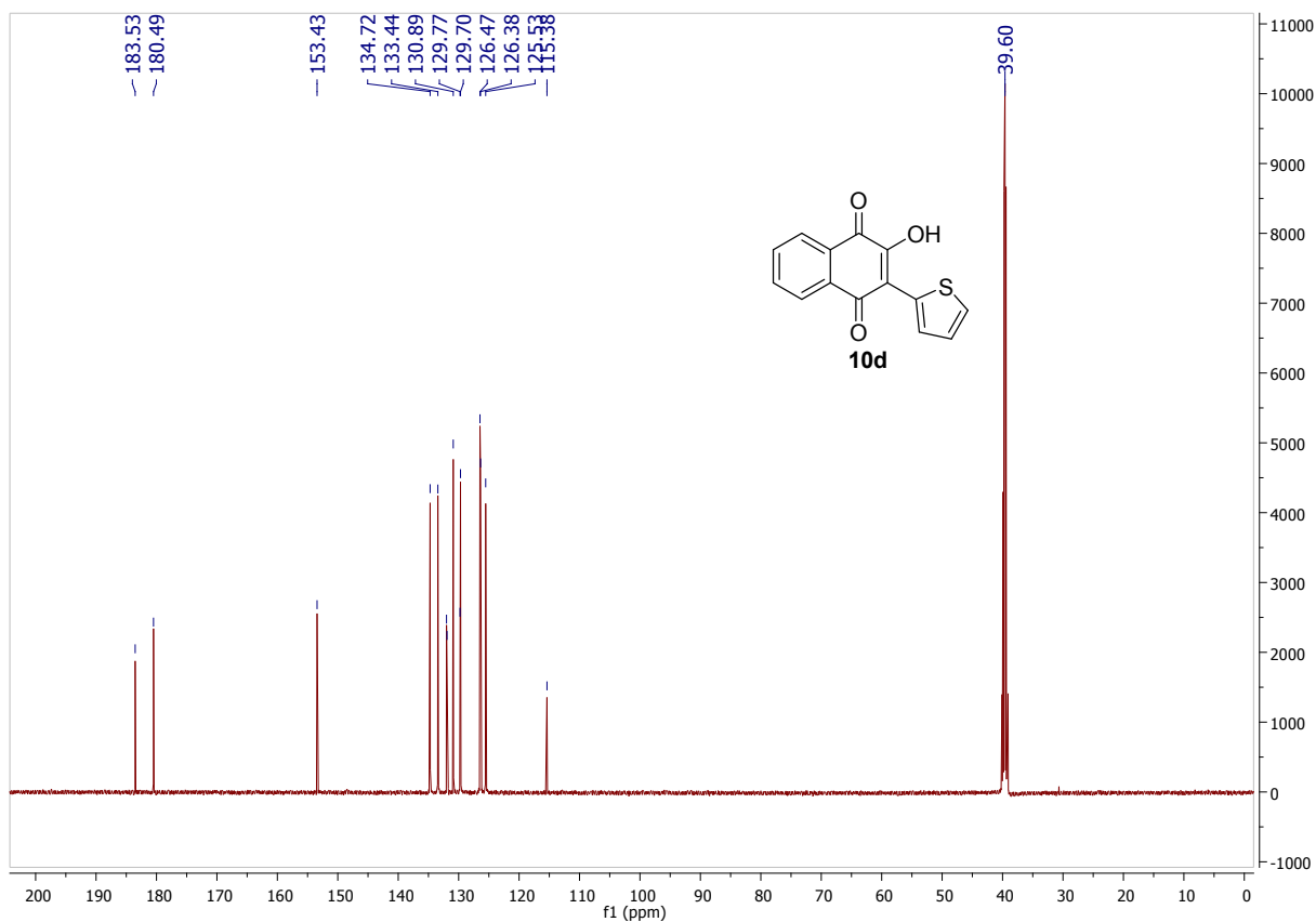
Figure S22 - 13 C NMR Spectra of 2-hydroxy-3-(thiophen-2-yl)naphthalene-1,4-dione ( 10d )
