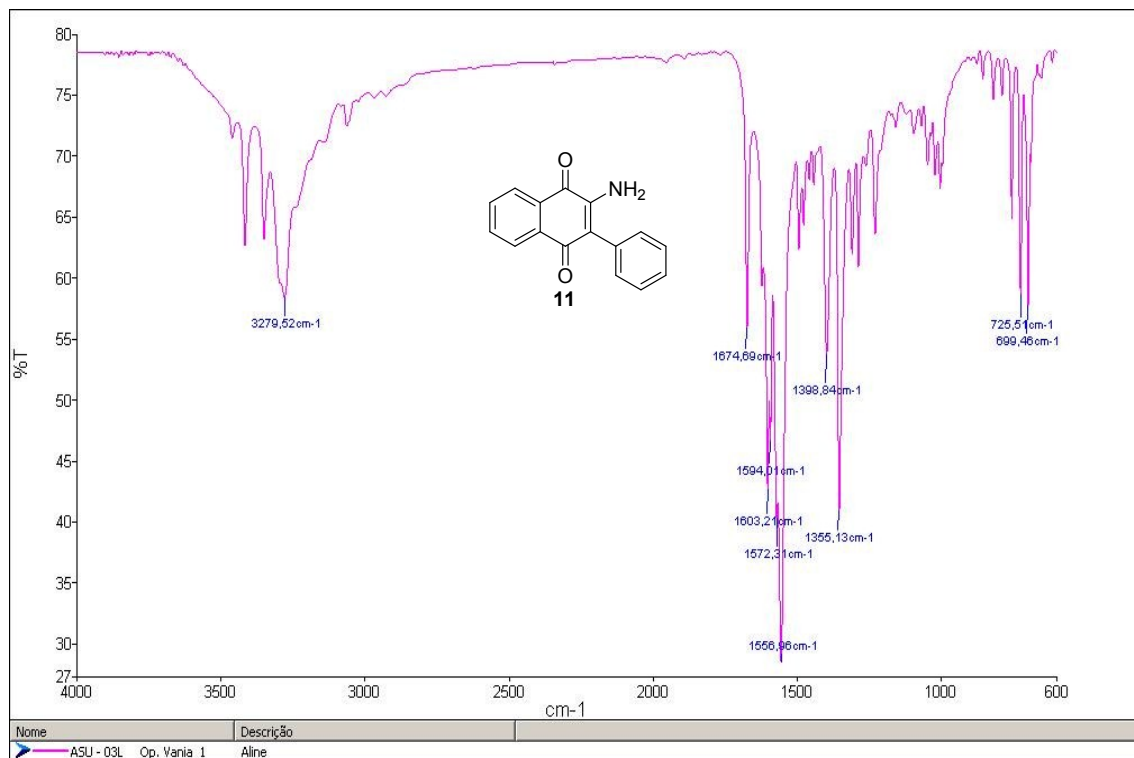
Figure S44 - Infrared spectrum of 2-amino-3-phenylnaphthalene-1,4-dione ( 11 )
