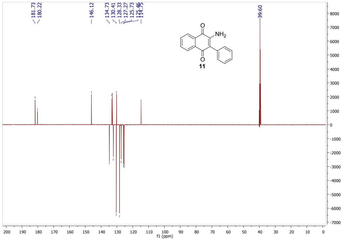
Figure S46 - ^{13}\text{C} NMR Spectra of 2-amino-3-phenylnaphthalene-1,4-dione ( 11 )
