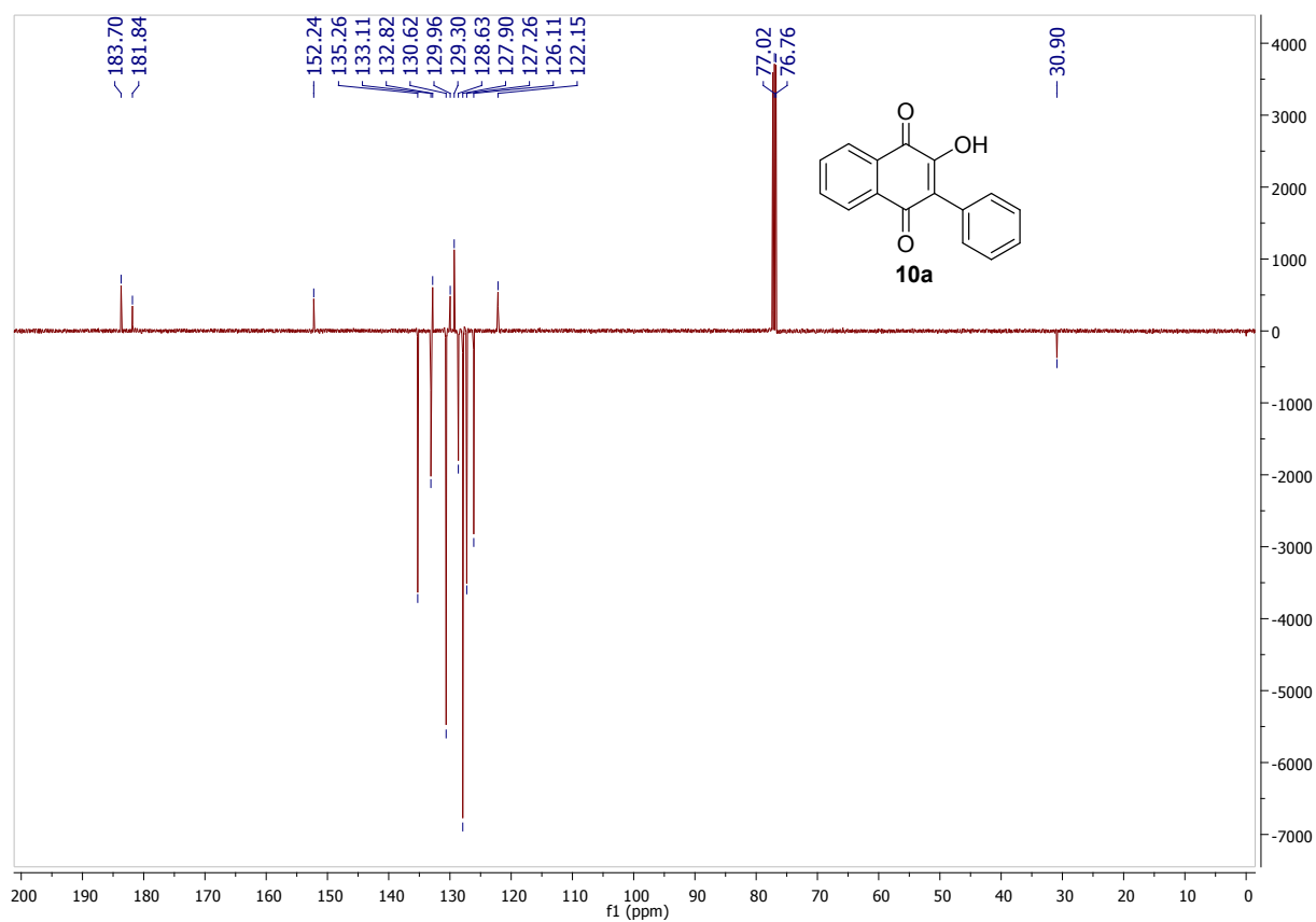
Figure S13 ^{13}\text{C} NMR Spectra of 2-hydroxy-3-phenylnaphthalene-1,4-dione ( 10a )
