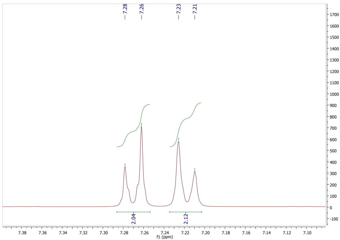
Figure S42 - ^1\text{H} NMR Spectra of 2-Hydroxy-3-( p -tolyl)naphthalene-1,4-dione ( 10k )
