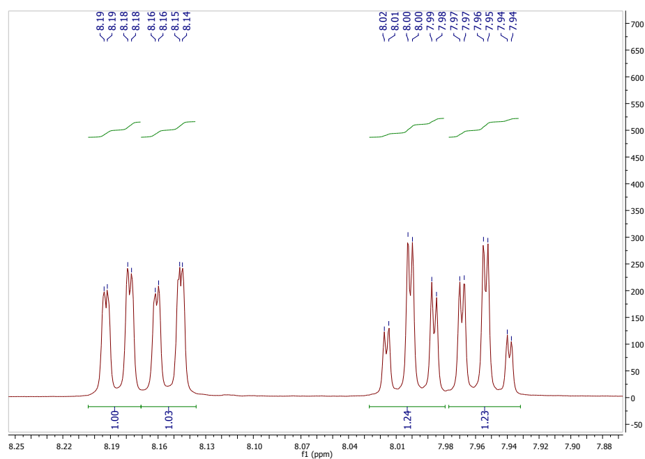
Figure S11 – ^1\text{H} NMR Spectrum of 2-hydroxy-3-phenylnaphthalene-1,4-dione ( 10a )
