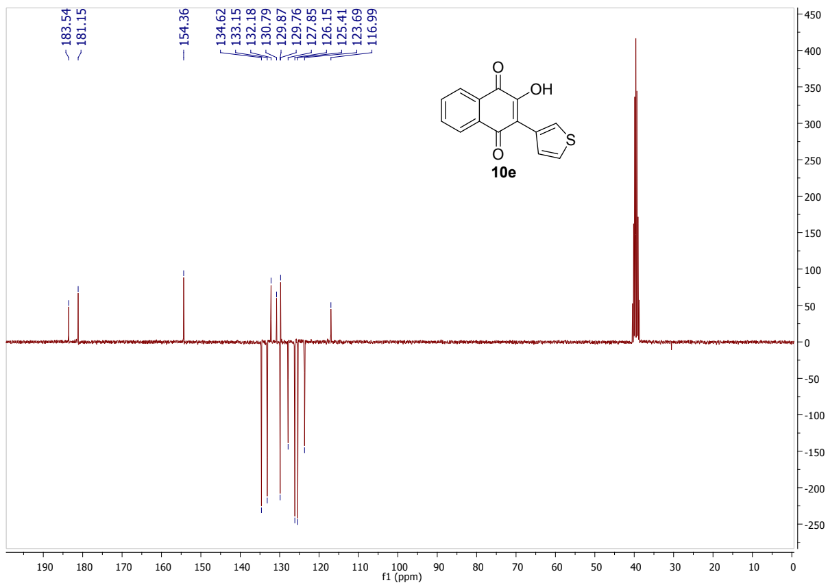
Figure S25 - ^{13}\text{C} NMR Spectra of 2-hydroxy-3-(thiophen-3-yl)naphthalene-1,4-dione ( 10e )
