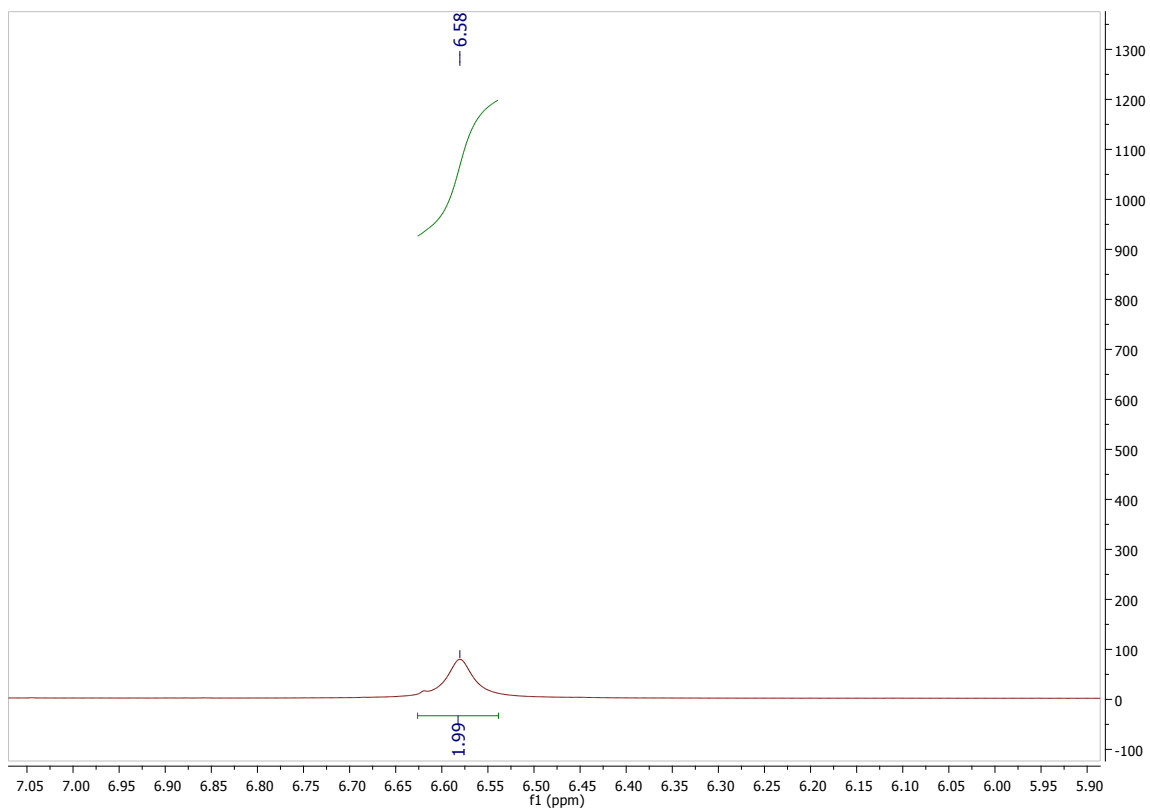
Figure S45 - ^1\text{H} NMR Spectra of 2-amino-3-phenylnaphthalene-1,4-dione ( 11 )
