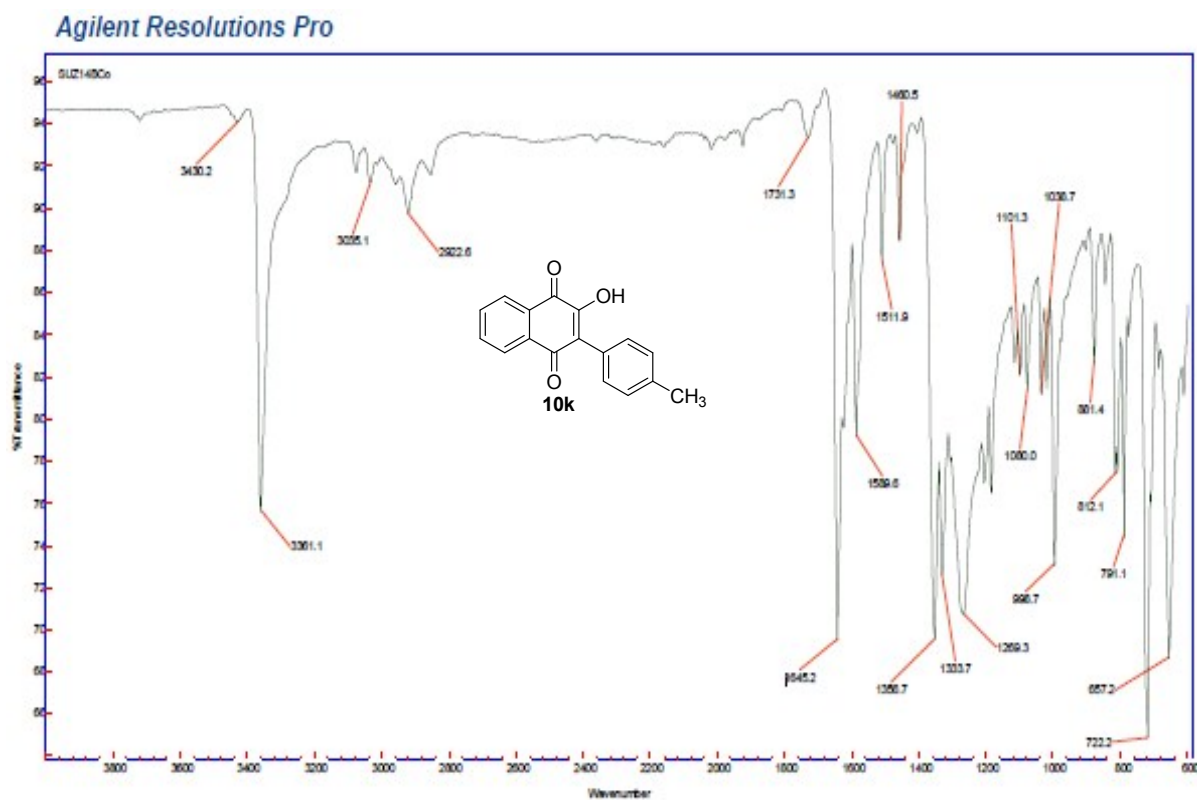
Figure S41 - Infrared spectrum of 2-Hydroxy-3-( p -tolyl)naphthalene-1,4-dione (10k)
