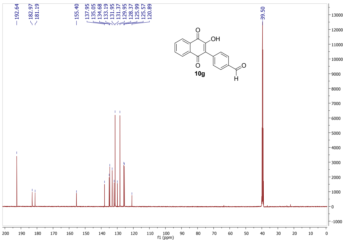
Figure S31 - ^{13}\text{C} NMR Spectra of 4-(3-hydroxy-1,4-dioxo-1,4-dihydronaphthalen-2-yl)benzaldehyde ( 10g )
