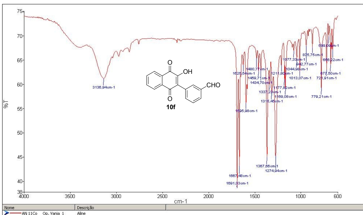
Figure S26 - Infrared spectrum of 3-(3-Hydroxy-1,4-dioxo-1,4-dihydronaphthalen-2-yl)benzaldehyde (10f)
