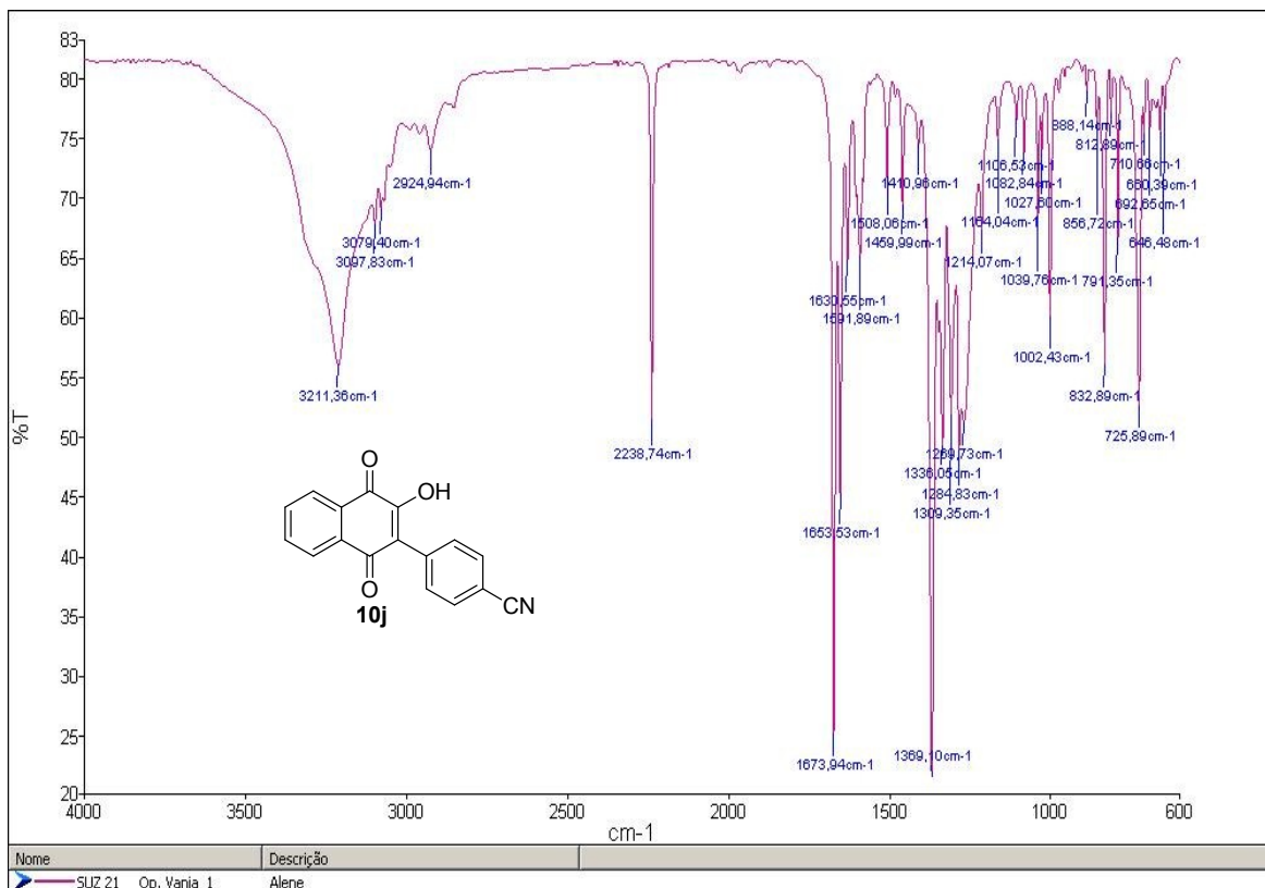
Figure S38 - Infrared spectrum of 4-(3-Hydroxy-1,4-dioxo-1,4-dihydronaphthalen-2-yl)benzotrile (10j)
