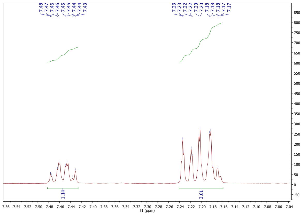
Figure S18 - ^1\text{H} NMR Spectra of 2-(3-fluorophenyl)-3-phenylnaphthalene-1,4-dione ( 10c )
