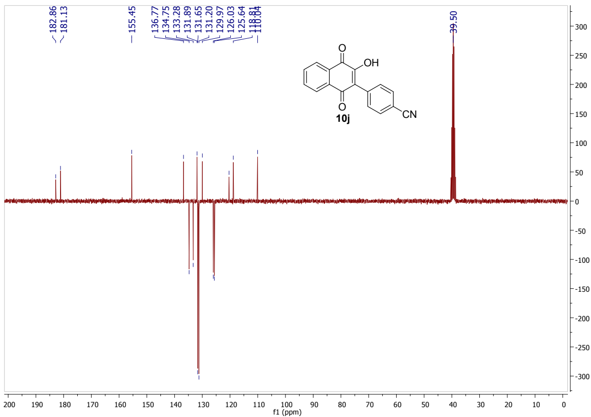
Figure S40 - ^{13}\text{C} NMR Spectra of 4-(1,4-dihydro-2-hydroxy-1,4-dioxonphtalen-3-yl)benzotrile ( 10j )
