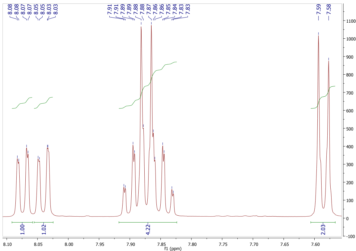
Figure S39 - ^1\text{H} NMR Spectra of 4-(3-Hydroxy-1,4-dioxo-1,4-dihydronaphthalen-2-yl)benzotrile ( 10j )
