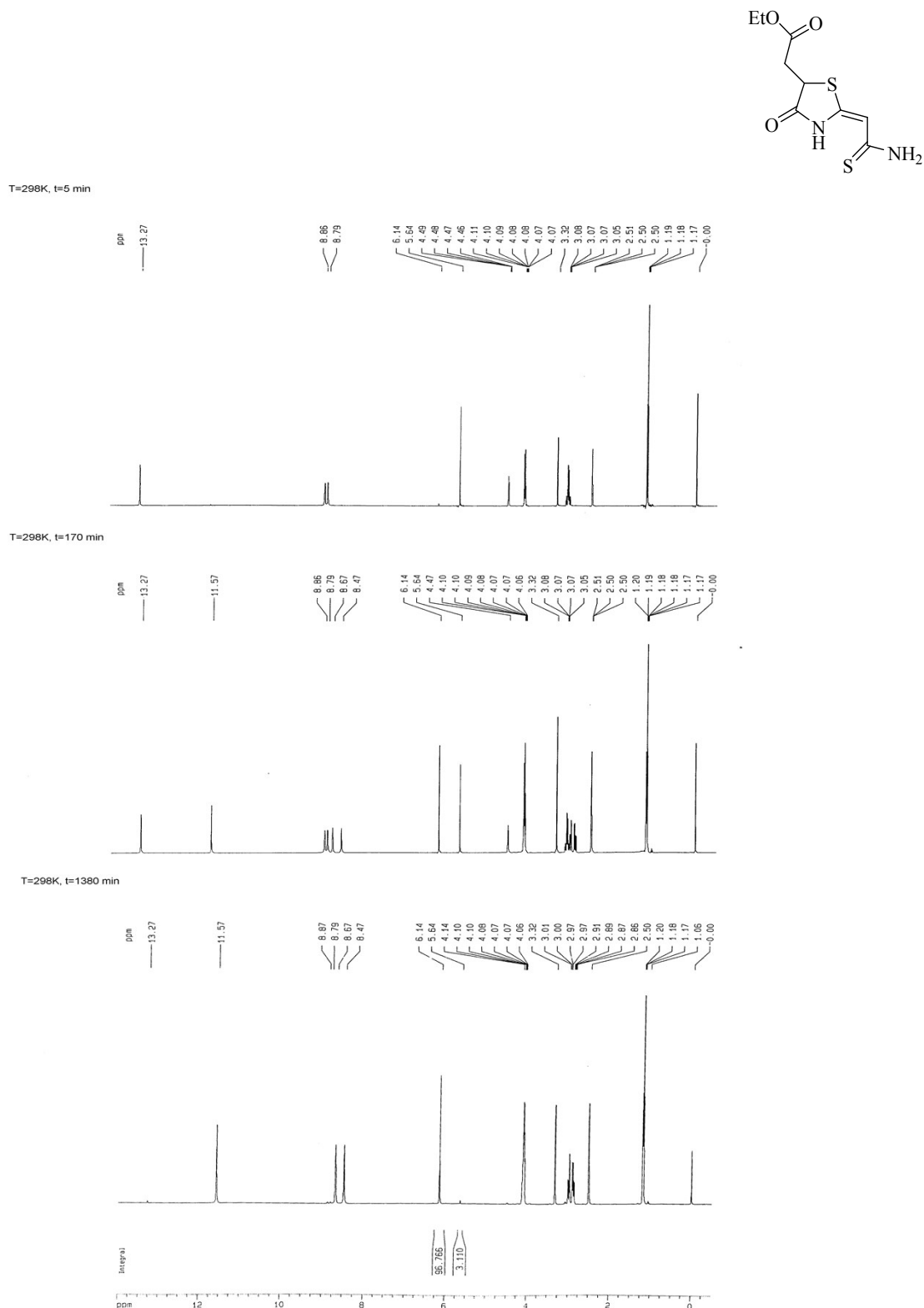
Figure S1. The facile E to Z isomerization of ( E )-(5-ethoxycarbonylmethyl-4-oxothiazolidin-2-ylidene)ethanthioamide 9a at 298 K illustrated by the three 1 H NMR spectra recorded 5, 170 and 1380 minutes after its dissolution (DMSO- d 6 )
