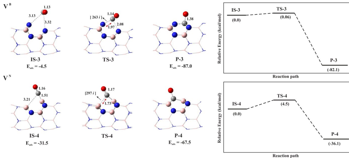
Figure S2. Optimized geometries of each step in the CO-vacancy recombination process over (5,0) BNNT. All energy values and distances are in kcal/mol and Å, respectively. For the transition state structures, the red arrow indicates the displacement vector along the imaginary frequency. The imaginary frequency value is shown within the bracket.
