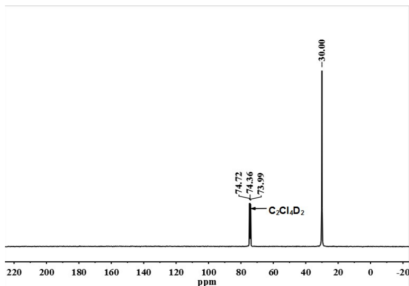
Fig. 2 † 13 C NMR spectra of the PE sample obtained in entry 23 in Table 7.
