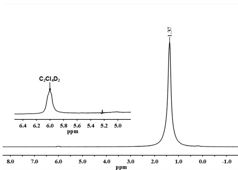
Fig. 1 † 1 H NMR spectra of the PE sample obtained in entry 23 in Table 7.
