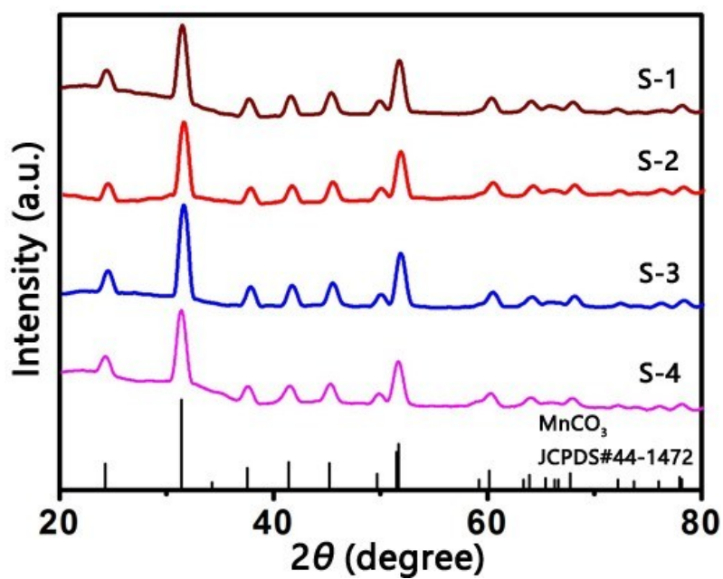
Fig. S1. The XRD patterns of S-1, S-2, S-3, and S-4.
