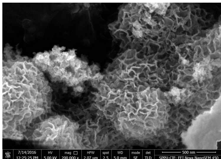
Fig. S1 SEM micrographs for the obtained nickel sulfide obtained from the precursor 1 .
