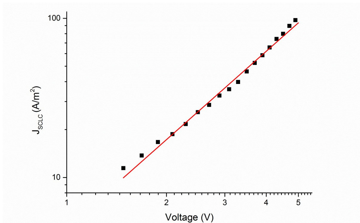
Dark I-V curve for HC61NP with linear fitting
