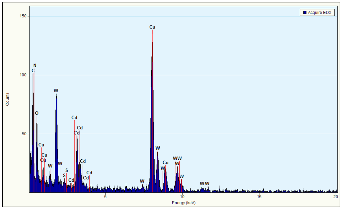
Fig. S2 EDX spectrum of 10CN-CSW core-shell photocatalyst.
