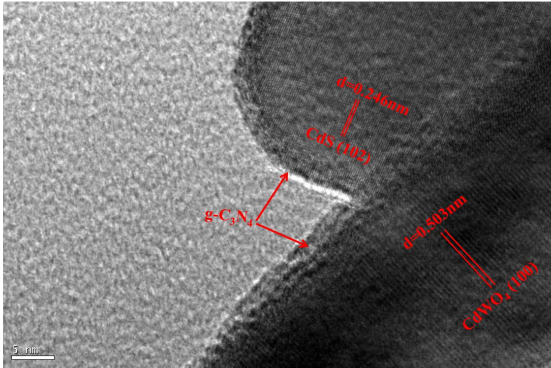
Fig. S1 HRTEM image of 10CN-CSW core-shell photocatalyst.
