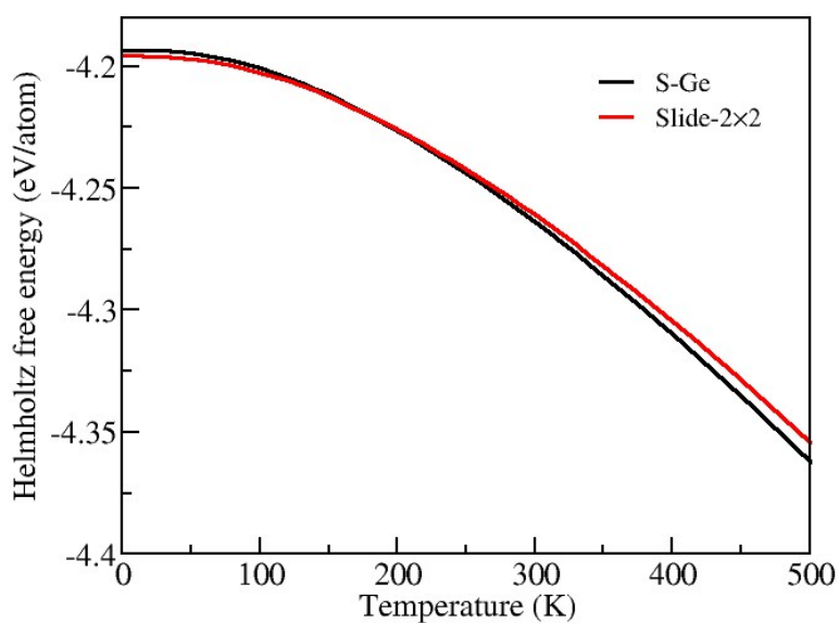
Fig. S1 Helmholtz free energy of S-Ge and slide-2×2 with respect to temperature.
