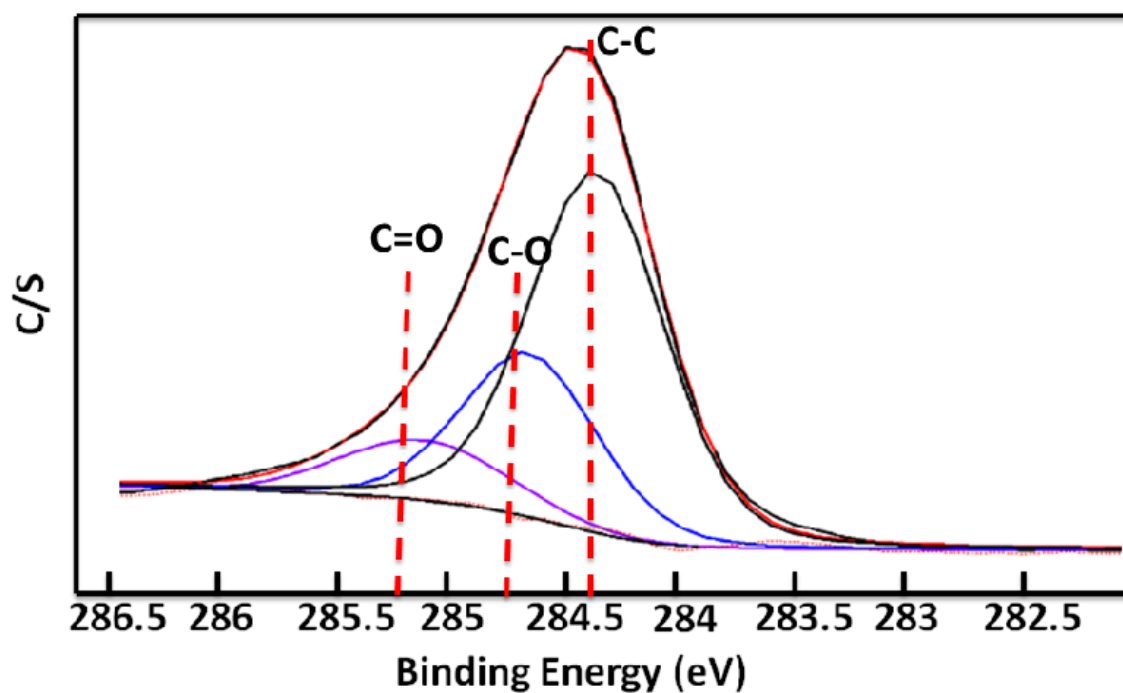
Supplementary Figure 3: XPS Spectrum of rGO-CNT foam. In high-resolution XPS analysis, the C-C and C-O bonds are at 284.4 and 284.7eV. The peak at 285.2 corresponds to C=O bonding.
