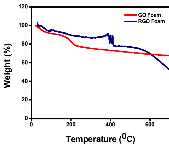
Supplementary Figure 2: TGA plots for GO and rGO foam showing substantial weight decrease for GO foam at 200 0 C while rGO foam shows gradual decomposition.
