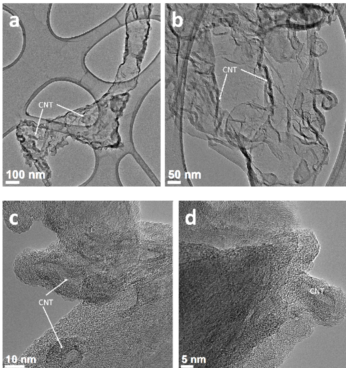
Supplementary Figure 1: (a,b) TEM of rGO-CNT foam showing CNT growth on rGO flakes (c,d) HRTEM of rGO-CNT foam showing CNT and rGO junctions.
