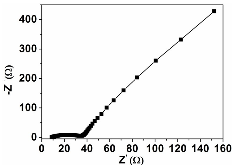
Fig.S2. Nyquist plot of PANI/Au/PC-100 after 2000th cycles
