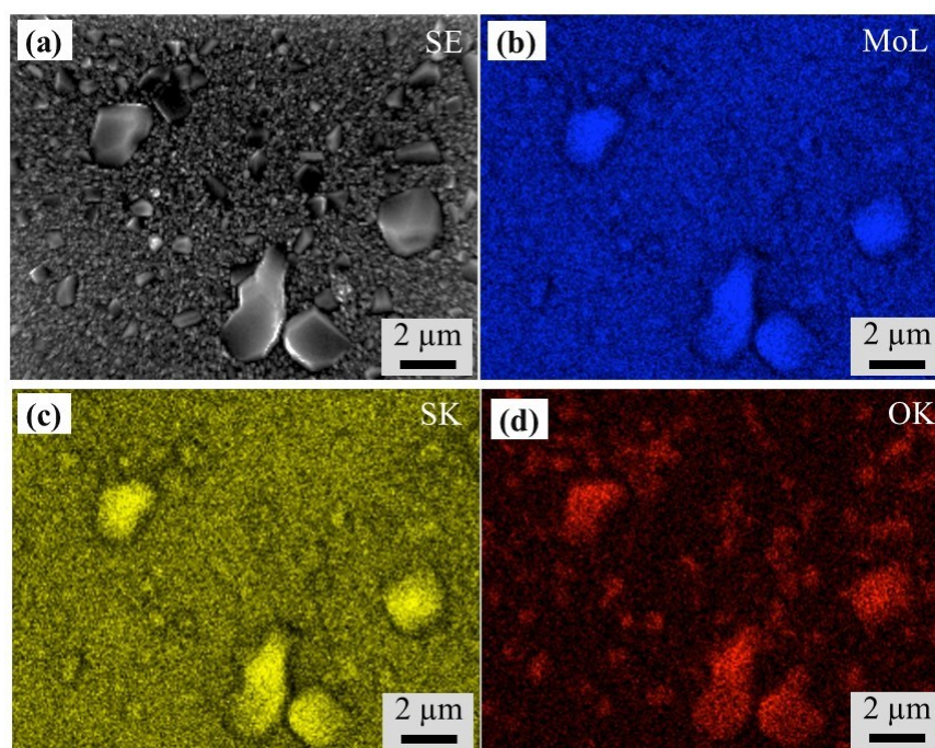
Figure S1 EDS map-scan of the sulfurized 50 nm Mo film surface, showing the elemental composition of the material.
