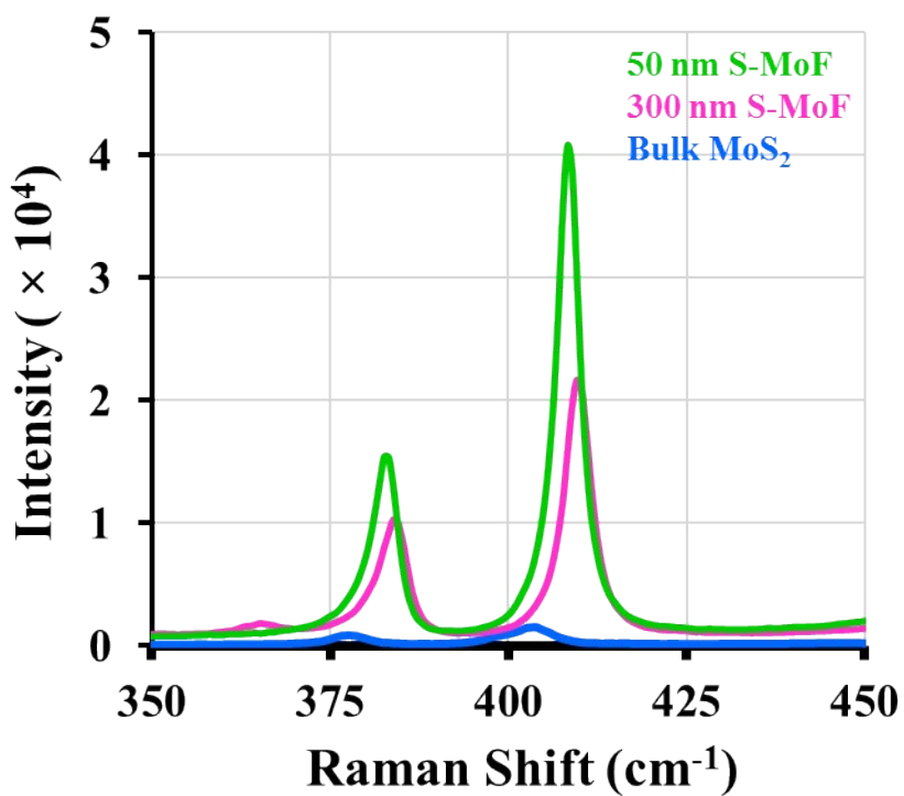
Figure S4 Raman spectra (acquisition time 60 s) for bulk, 300 nm S-Mo and 50 nm S-Mo samples indicating one order of magnitude enhancement in the A 1g mode for the NSs samples as compared to the bulk MoS 2
