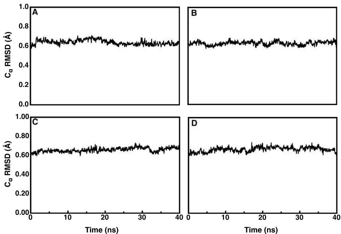
Figure S2: Plots of the RMSD of all backbone C_{\alpha} atoms during the equilibration of the R-C1B1 variant of StEH1 in complex with (A,B) ( R )- and (C,D) ( S )-SO bound in Mode1 and Mode2 respectively (for a definition of the two binding modes see Figure 4 of the main text). RMSD plots are shown in Å, relative to the original crystal structure.
