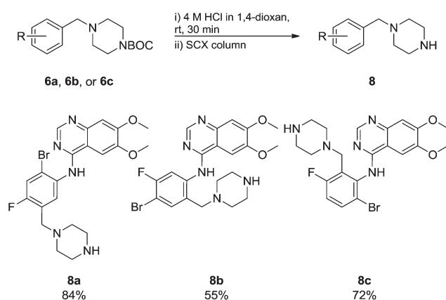
Scheme 8 Boc cleavage.
