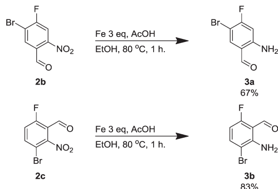
Scheme 1 Iron-mediated reductions of compounds 2b and 2c.
