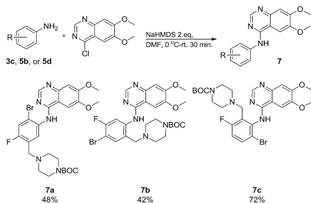
Scheme 7 Linking of the quinazoline unit.
