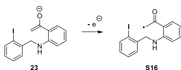
SM (Before SET): 23 in Benzene
