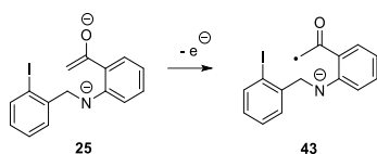
SM (Before SET): 25 in Benzene
