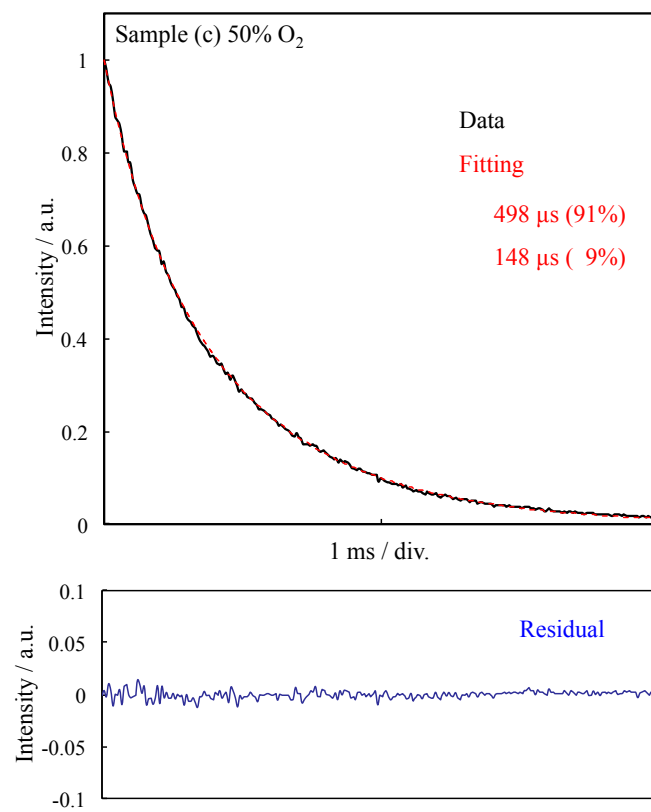
Figure S1. Fitting of lifetime measurement for sample (c) at 50% O 2 concentration.
