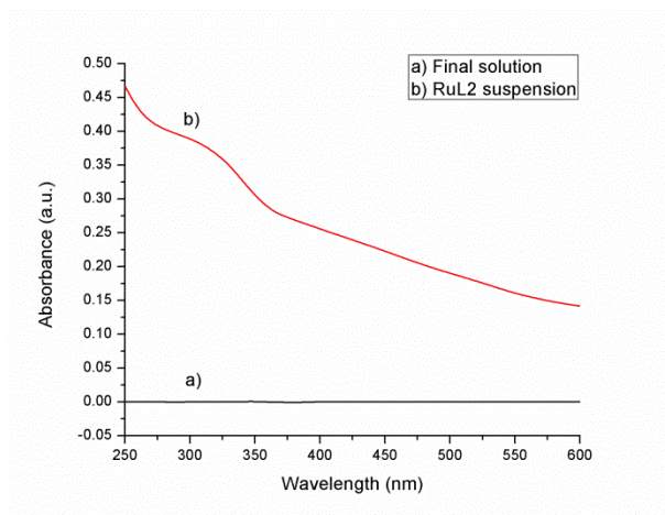
Figure SM1. Comparison of the UV-Vis spectra of: a) final solution obtained when RuL2-TiO 2 catalyst was vigorously stirred under visible light during 5 h and b) an aqueous suspension of RuL2 complex ( 1 \times 10^{-5} M).
