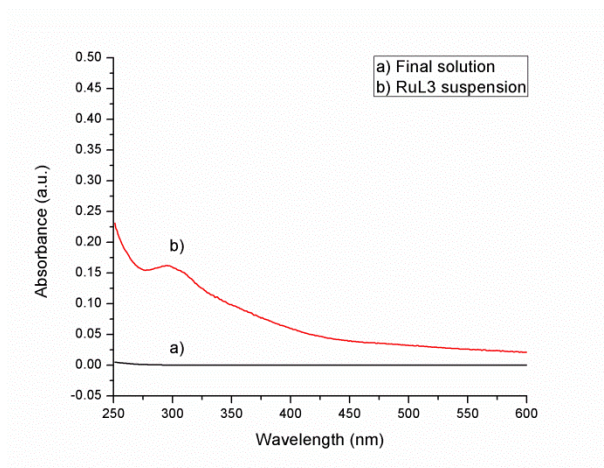
Figure SM2. Comparison of the UV-Vis spectra of: a) final solution obtained when RuL3-TiO 2 catalyst was vigorously stirred under visible light during 5 h and b) an aqueous suspension of RuL3 complex ( 1 \times 10^{-5} M).
