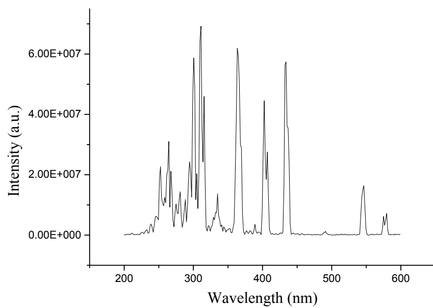
Fig. S2 Spectral irradiance of mercury lamp.
