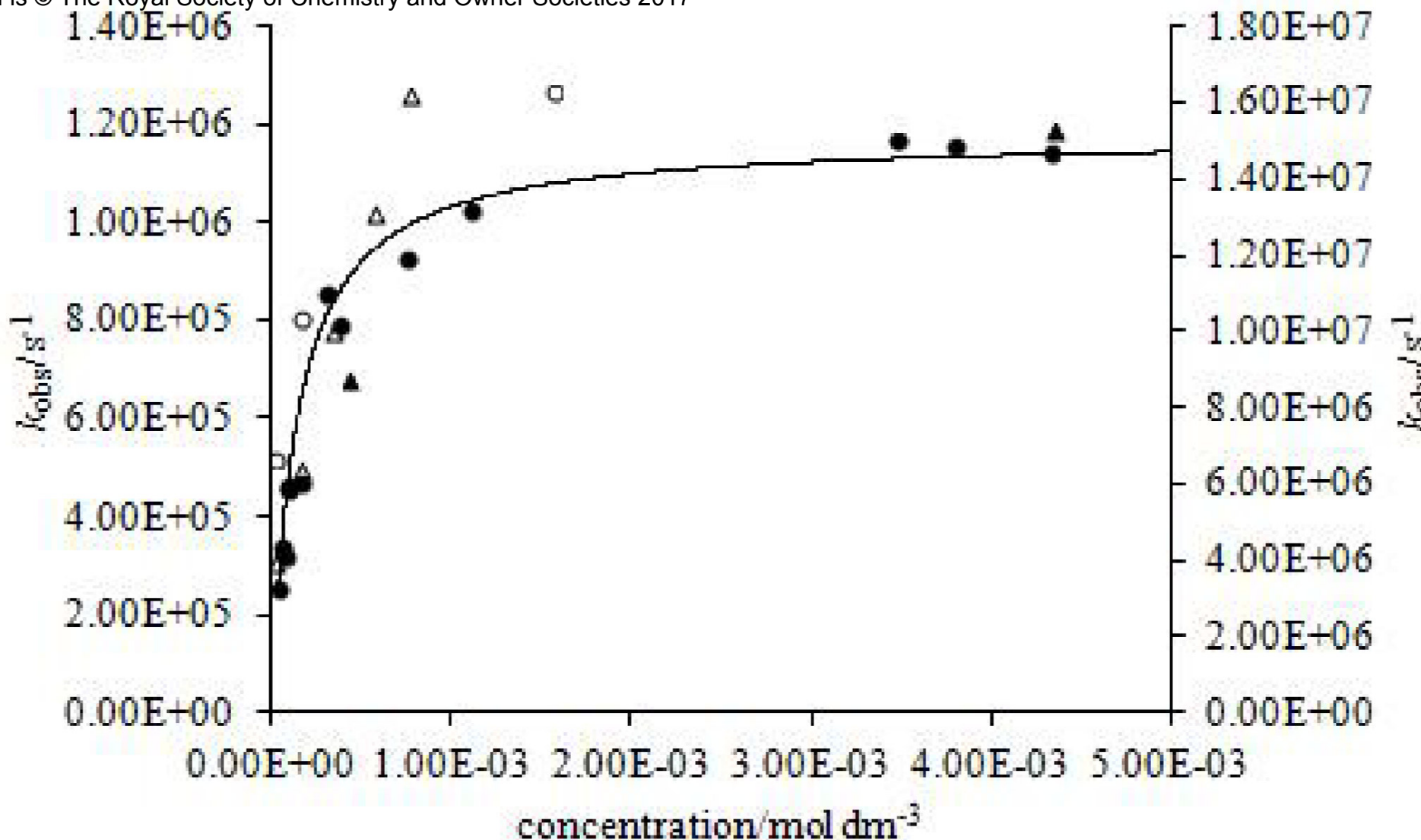
Fig. ESI1 Dependence of the first-order rate constant ( k_{\text{obs}} ) for the decay of ^3\text{NFA}^* on ground-state concentration of NFA, in acetonitrile ( \bullet ), in acetone ( \Delta ), in 1,4-dioxane ( \circ ) and in hexane ( \blacktriangle ). ( k_{\text{obs}} values in hexane refer to scale on the right-hand side)
