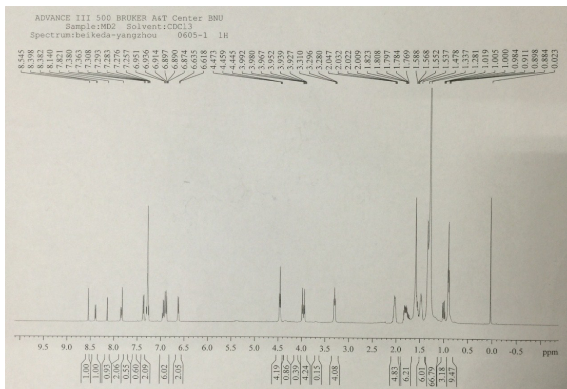
Fig. S1. ^1\text{H} NMR spectra of MD1 .
