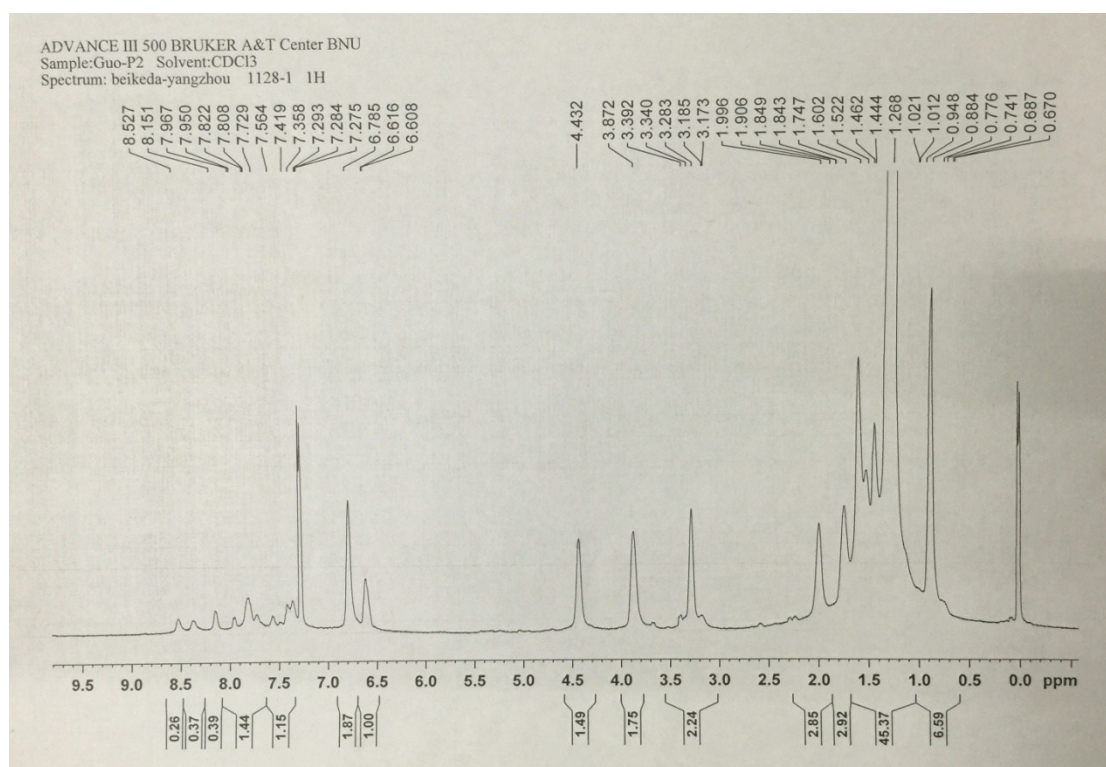
Fig. S3. 1 H NMR spectra of P1 .
