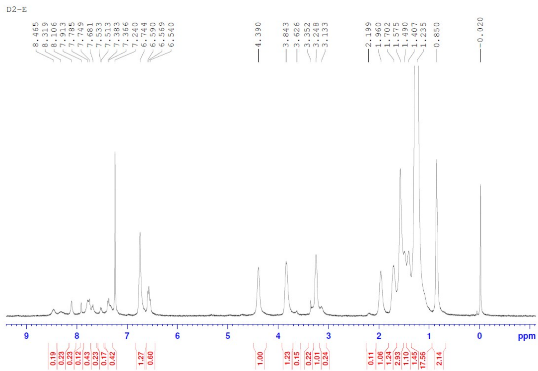
Fig. S4. ^1\text{H} NMR spectra of P2 .
