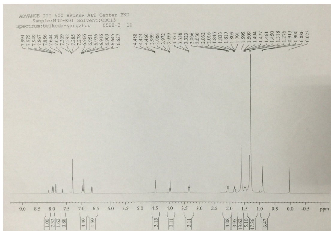
Fig. S2. ^1\text{H} NMR spectra of MD2.
