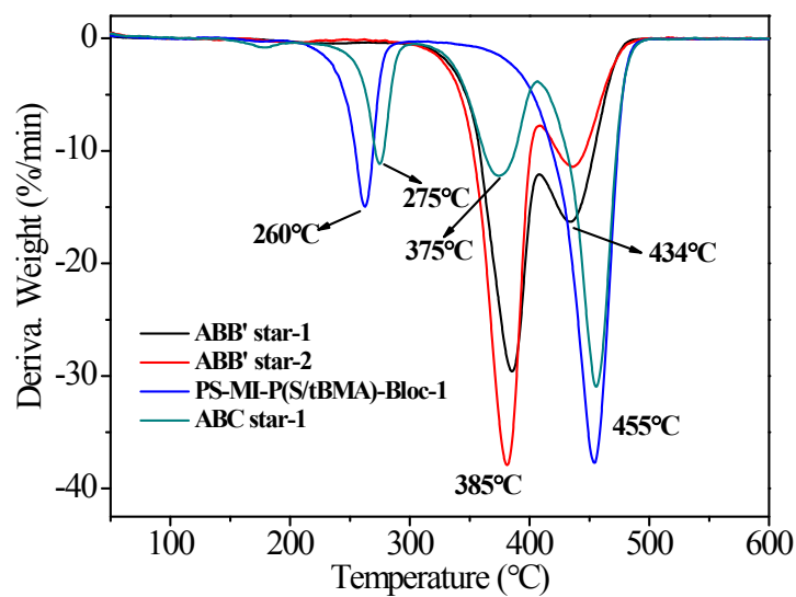
Figure S3. DTG traces of PS-MI-P(S/tBMA)-Bloc-1, ABB' star-1, ABB' star-2 and ABC star-1.
