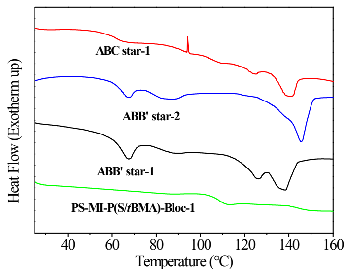
Figure S4. DSC curves of PS-MI-P(S/tBMA)-Bloc-1, ABB' star-1, ABB' star-2 and ABC star-1 (first heating process).
