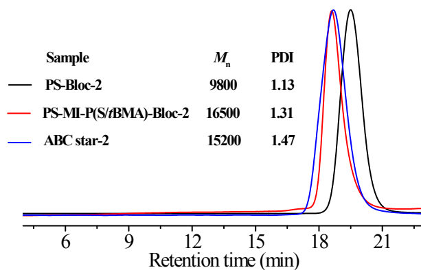
Figure S2. GPC traces of PS-Bloc-2, PS-MI-PS'-Bloc-2 and ABC star-2.
