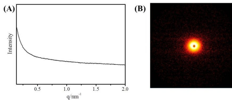
Figure S5. (A) 1D SAXS and (B) 2D SAXS profiles of ABB' star-1.
