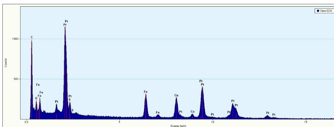
Figure S1 EDX spectrum of the resultant FePt-1 NPs.
