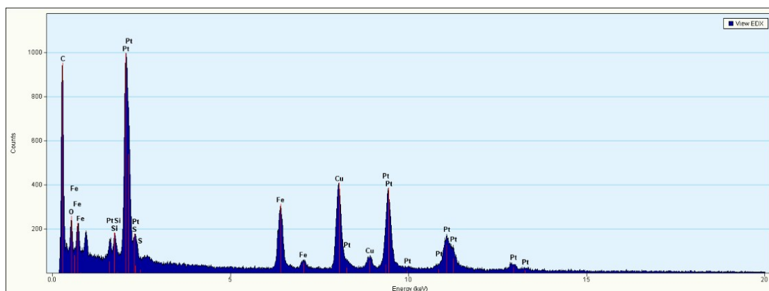
Figure S2 EDX spectrum of the resultant FePt-2 NPs.
