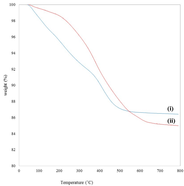
Fig. S1 TGA of (i) SNPs, (ii) SNPs-CTMS
