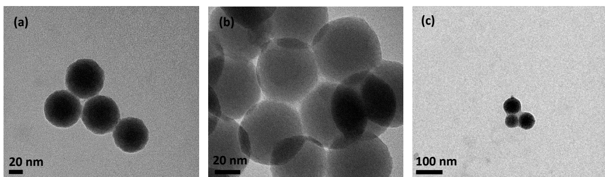
Fig. S3 TEM images of (a) PSNP-B-I, (b) PSNP-B-II (c) PSNP-B-III
