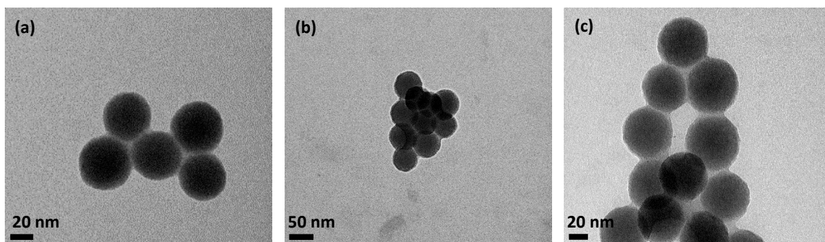
Fig. S2 TEM images of (a) PSNP-A-I, (b) PSNP-A-II (c) PSNP-A-III
