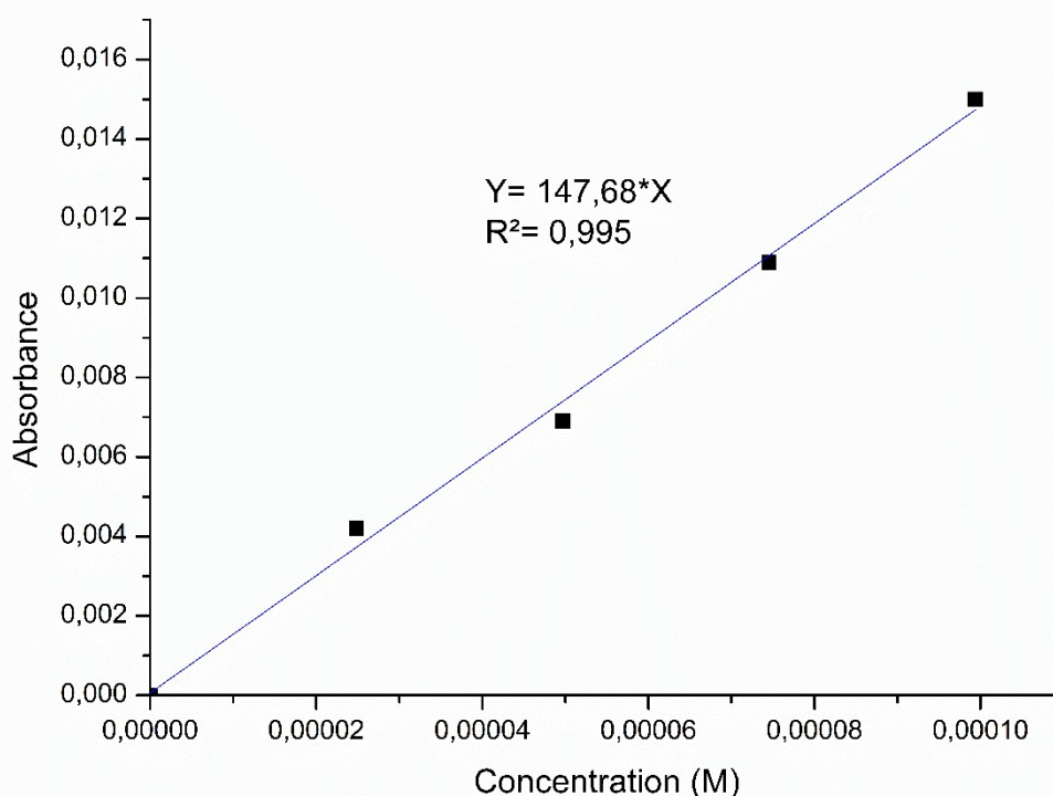
Figure 1 : UV absorbance evolution with 4-Phenyl-1,2,4-triazoline-3,5-dione (PTAD) concentration at 540 nm
