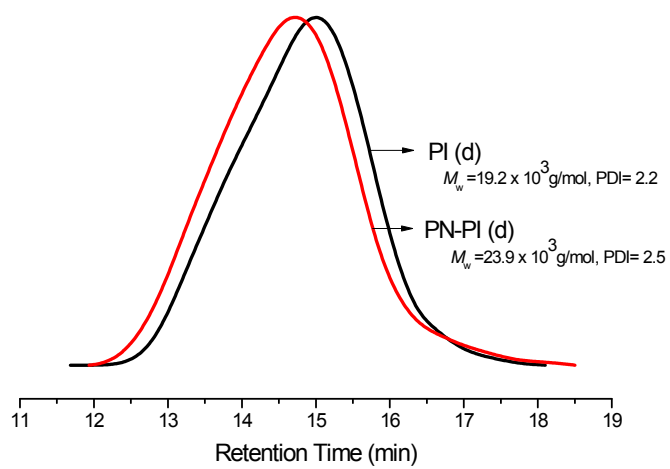
Fig. S2. GPC curves of PI (c, d) and PN-PI (c, d)
