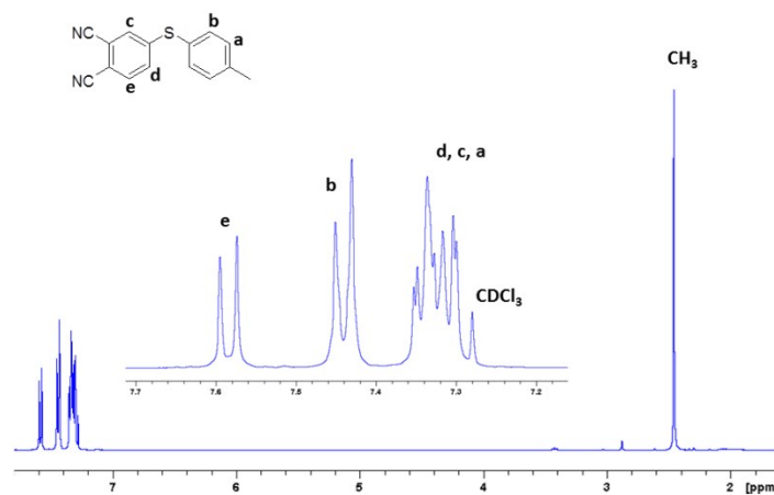
Figure S1. ^1\text{H} NMR spectrum of model compound 1 in \text{CDCl}_3
