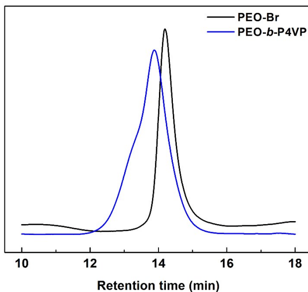
Figure S2 GPC curves of macro-initiator PEO-Br and diblock copolymer PEO- b -P4VP
