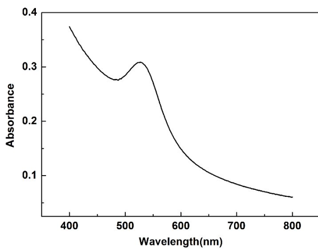
Figure S5 UV-vis spectrum of YSNs in water
