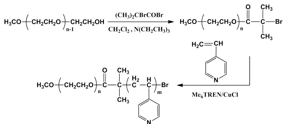
Figure S1 The synthesis route for diblock copolymer PEO- b -P4VP
