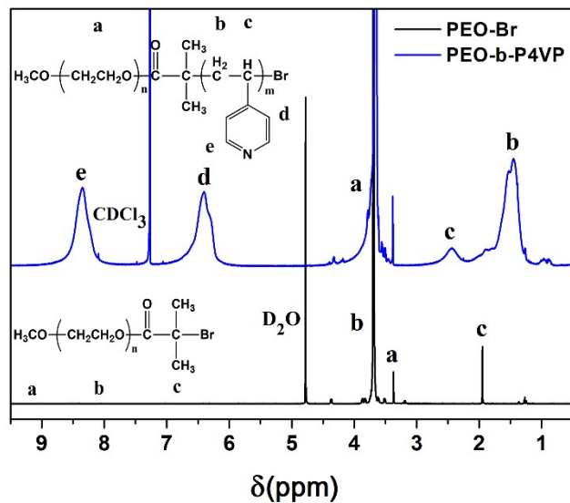
Figure S3 ^1\text{H} NMR spectra of macro-initiator PEO-Br and diblock copolymer PEO-b-P4VP
