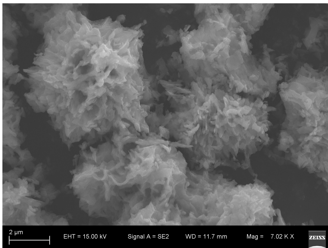
Fig. S3 The SEM image of the samples obtained after the 10000 cycle life testing.
