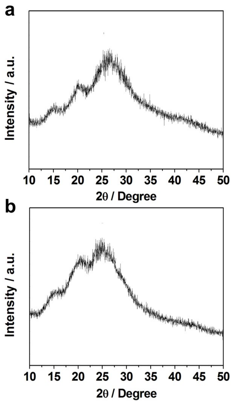
Fig. S2 The XRD patterns of the samples of sample which was modified by SDS (a) and CTAB (b), other conditions are the same as the PVP.
