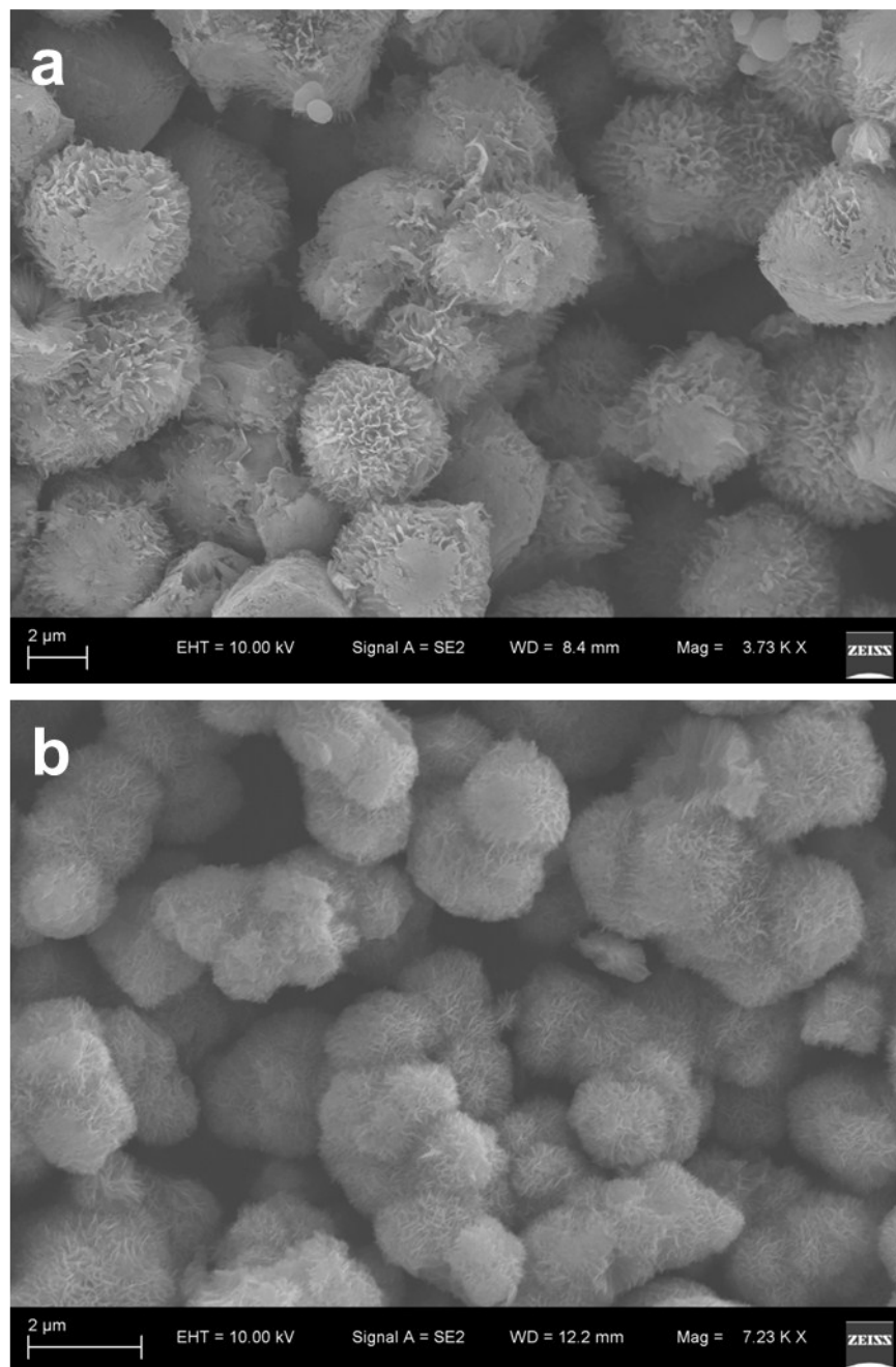
Fig. S1 The FRSEM images of the samples of sample which was modified by SDS (a) and CTAB (b), other conditions are the same as the PVP.
