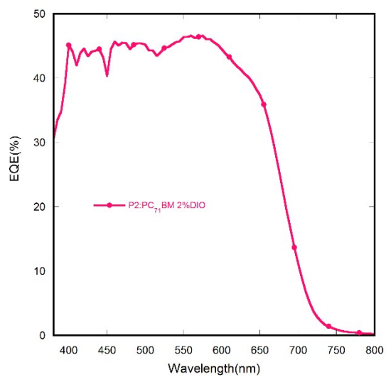
Figure S2. EQE spectra of P2:PC 71 BM based device with 2%DIO.
