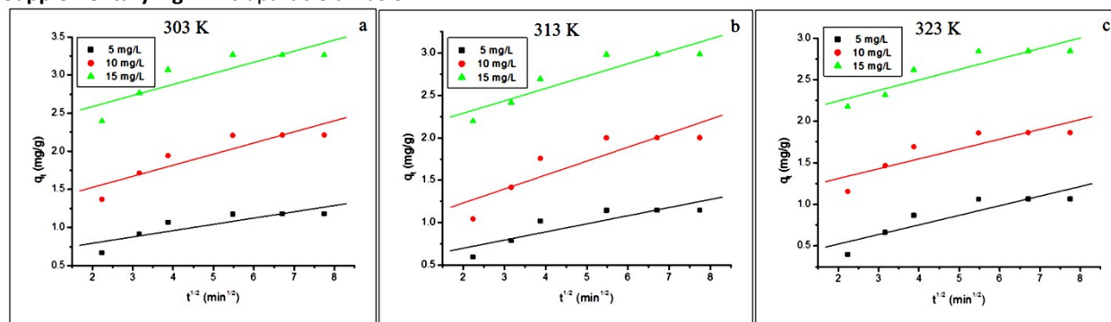
Supplementary Fig. 4 Intraparticle diffusion.
