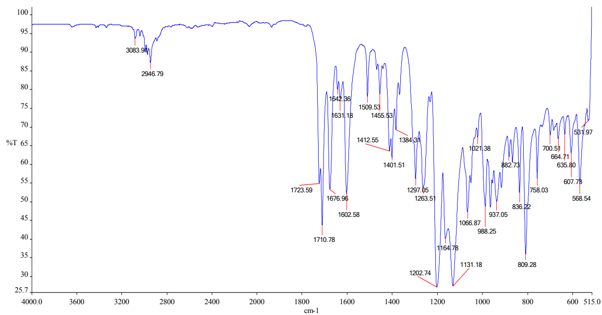
Figure 1s. FT-IR spectrum of diacrylated Irgacure-2959 (DAI).
