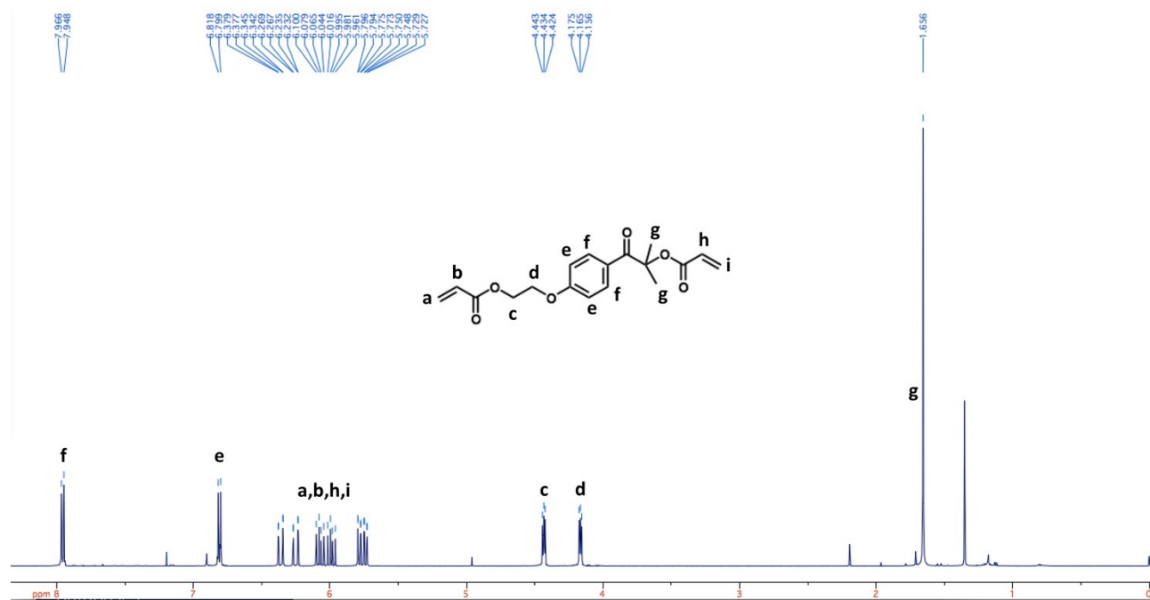
Figure 2s. ^1\text{H} NMR spectrum of diacrylated Irgacure-2959 (DAI) in \text{CDCl}_3 .
