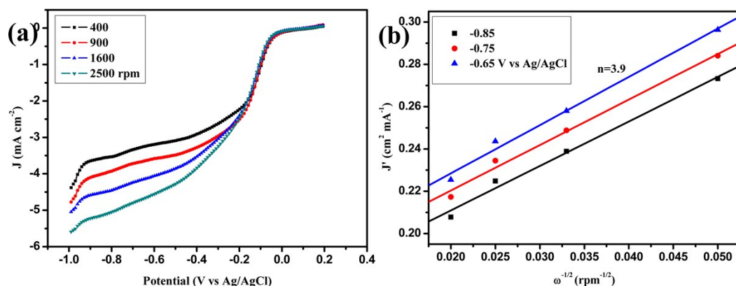
Figure S1. (a) RDE polarization curves at different rotation rates for ORR on GC with predeposited Pt/C in a 0.1 M KOH solution saturated with oxygen at the scan rate of 20 mV s -1 . (b) Plot of J^{-1} vs \omega^{-1/2} for oxygen reduction on GC with precoated Pt/C at potentials -0.65, -0.75 and -0.85V.
