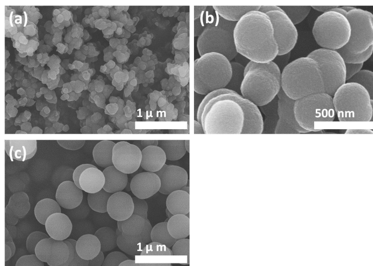
Fig. S1 SEM images of PDA particles prepared at the pH of (a) 7.5, (b) 8.0 and (c) 9.0.
