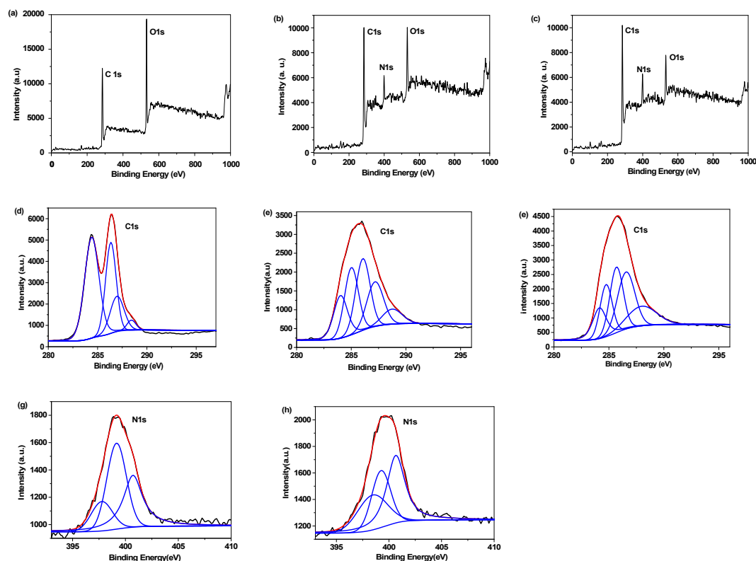
Fig. S1 XPS spectra of (a) GO, (b) GO/TAP, and (c) GOTAP; High-resolution XPS spectra in the C1s region of (d) GO, (e) GO/TAP, and (f) GOTAP; High-resolution XPS spectra in the N1s region of (g) GO/TAP and (h) GOTAP.
