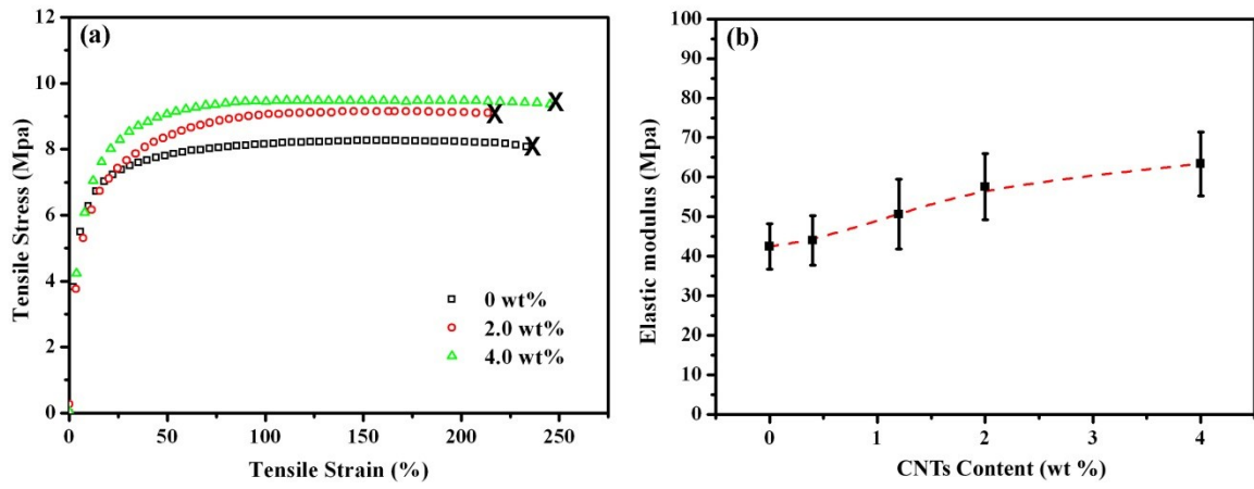
Fig. S3. Tensile properties for the CNTs/TPV composites with different CNTs contents: (a) the stress-strain curves for the composites; (b) the variation of the elastic modulus with the change in CNTs contents
