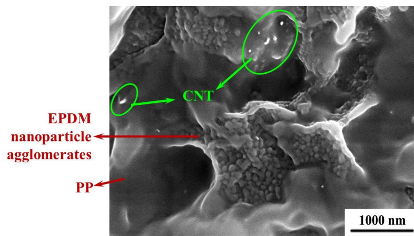
Fig. S1. SEM micrographs of CNTs/TPV composites with 0.5 wt% of CNTs
