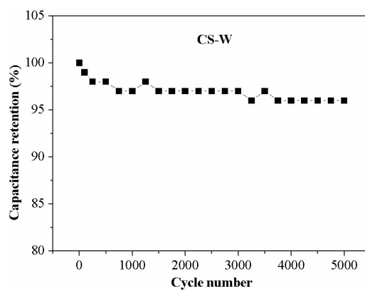
Figure S1. Cycling performance of CS-W at 1.0 A/g over 5000 cycles.
