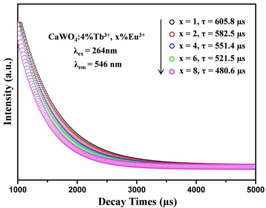
Fig. S2 Photoluminescence decay curves of \text{Tb}^{3+} in \text{CaWO}_4:4\%\text{Tb}^{3+}, x\%\text{Eu}^{3+} with changing \text{Eu}^{3+} concentrations.
