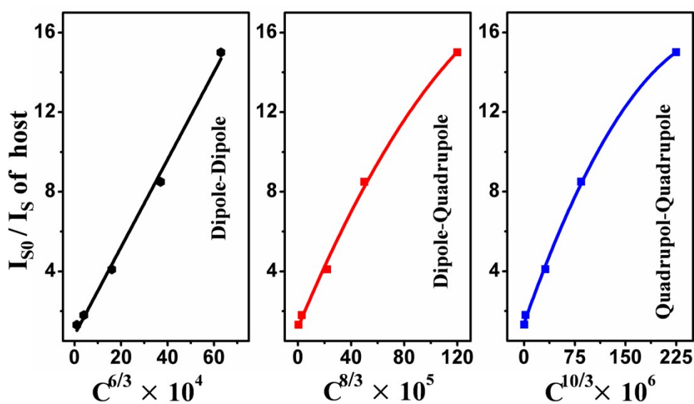
Fig. S1 Dependence of I_{S0}/I_S of host emission on (a) C_{\text{Tb}}^{6/3} , (b) C_{\text{Tb}}^{8/3} , and (c) C_{\text{Tb}}^{10/3} .
