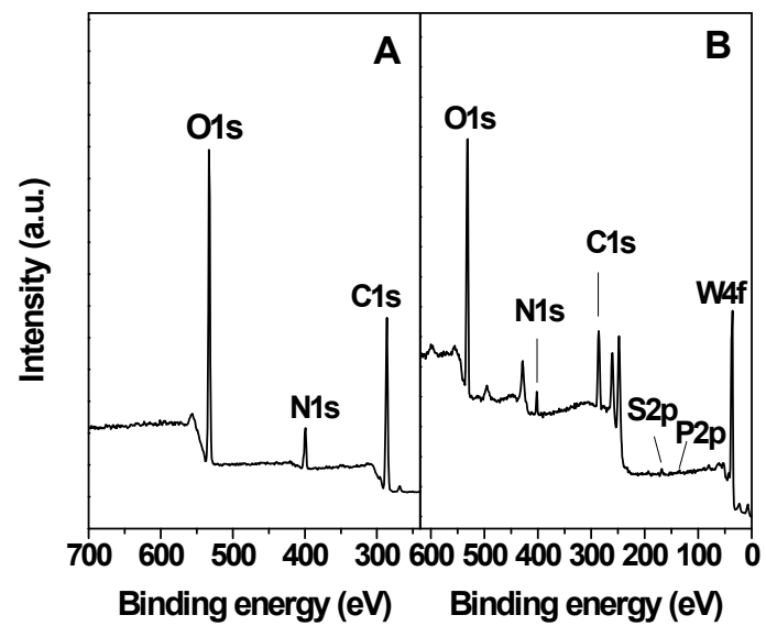
Fig. S1 XPS survey of (A) chitosan and (B) CS-VImPS-PW materials.
