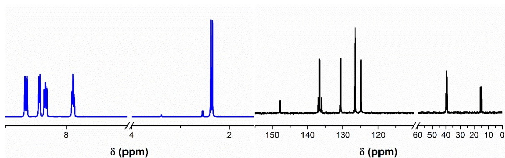
FIG. S2. ^1\text{H} NMR (blue) and ^{13}\text{C} NMR (black) spectra of DNMPPO.
