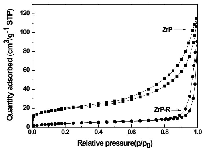
Fig.S1 The nitrogen adsorption and desorption isotherm of ZrP and ZrP-R.
