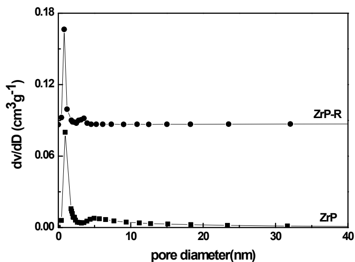
Fig. S2 Pore size distribution curves of ZrP and ZrP-R.
