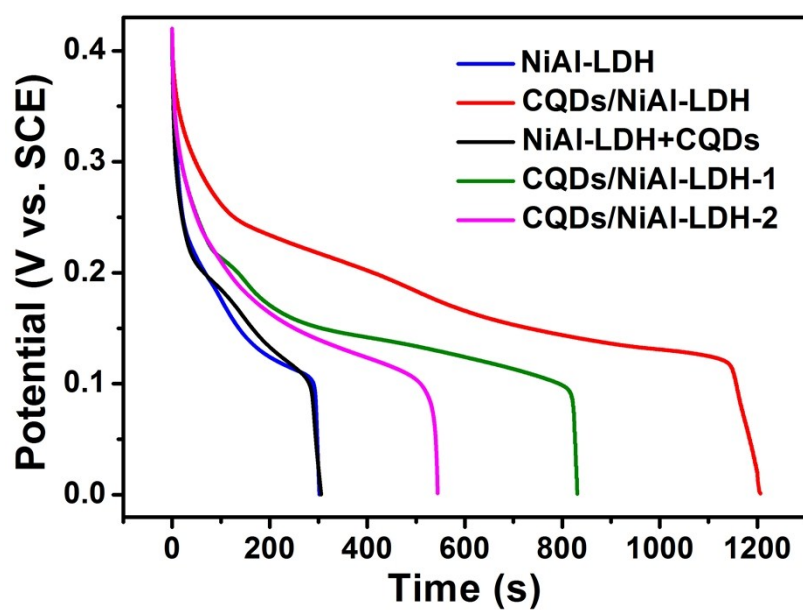
Fig. S3 The discharge curves of NiAl-LDH, CQDs/NiAl-LDH, NiAl-LDH+CQDs, CQDs/NiAl-LDH-1 and CQDs/NiAl-LDH-2 composites at current densities of 2 \text{ A g}^{-1} in 6 M KOH aqueous solution.
