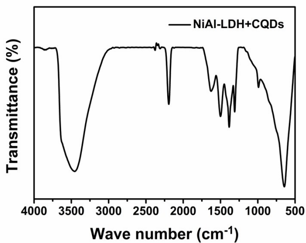
Fig. S2 FT-IR spectra for NiAl-LDH+CQDs.
