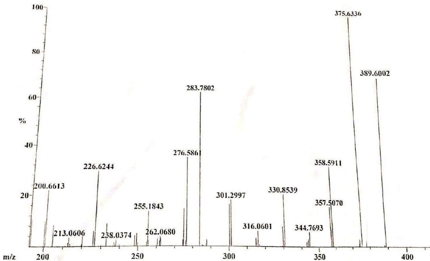
EI-MS spectra of DDPC.
