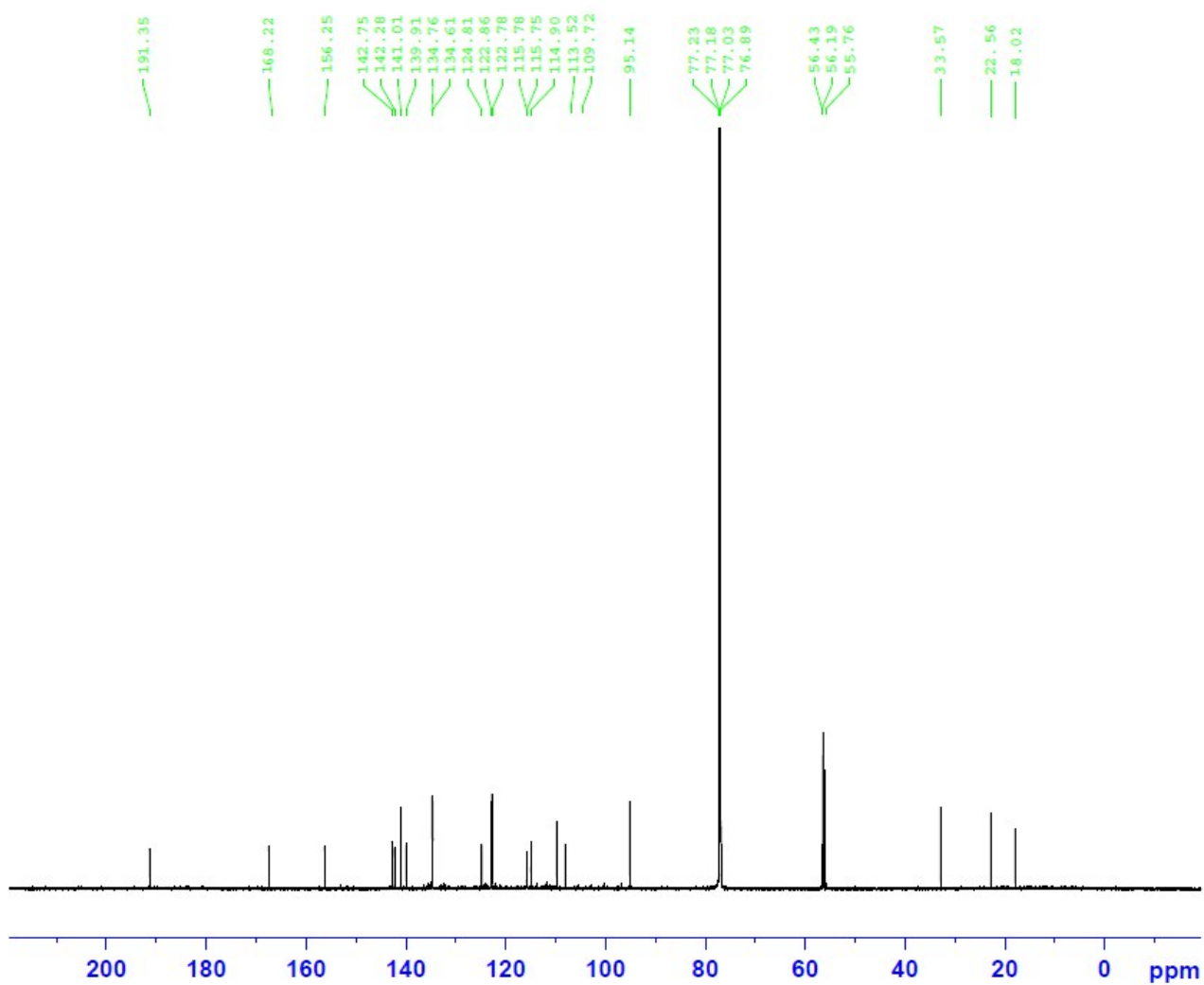
13C NMR spectra of DDPG.
