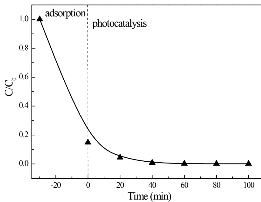
Fig S1. The adsorption ability and photocatalytic performance of TNTs/Fe 3 O 4 /GN composites for Rhodamine B
