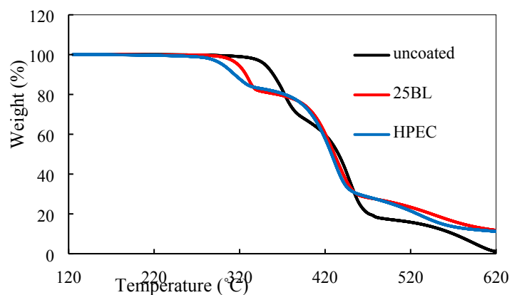
Fig. S2. Representative TGA weight loss, as a function of temperature, in oxidizing atmosphere.
