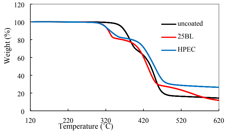
Fig. S3. Representative TGA weight loss, as a function of temperature, of uncoated and coated PECO fabrics in nitrogen atmosphere.
