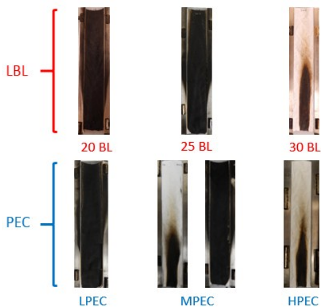
Fig. S1. Images of coated fabric residues after vertical flame testing.
