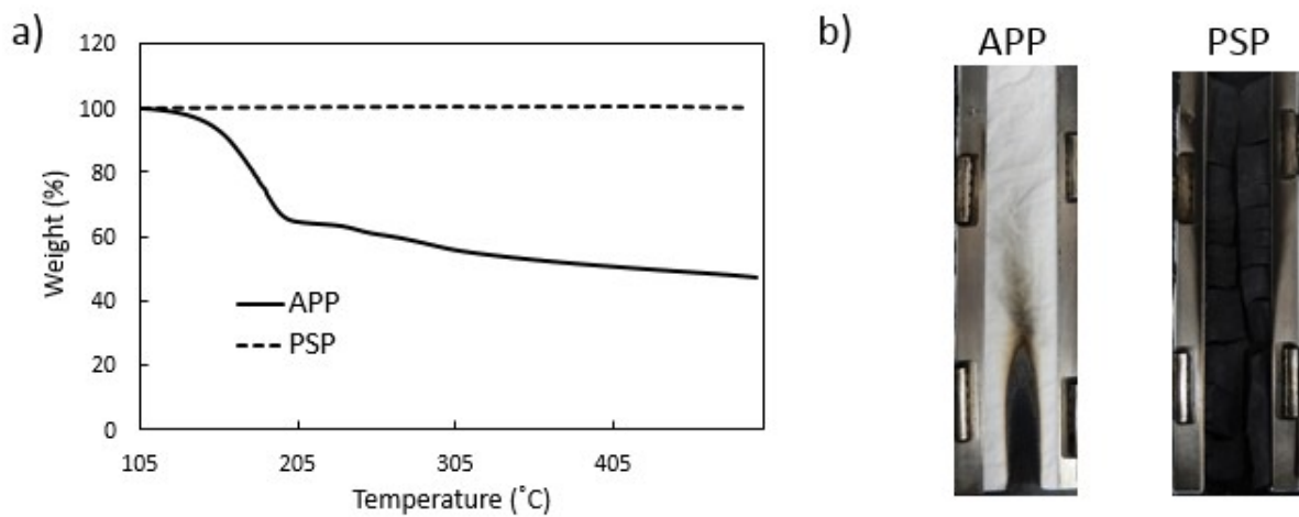
Fig. S4. Thermogravimetric analysis of ammonium polyphosphate (APP) and poly(sodium phosphate) PSP (a). APP and PSP-coated PECO after vertical flame testing (b).
