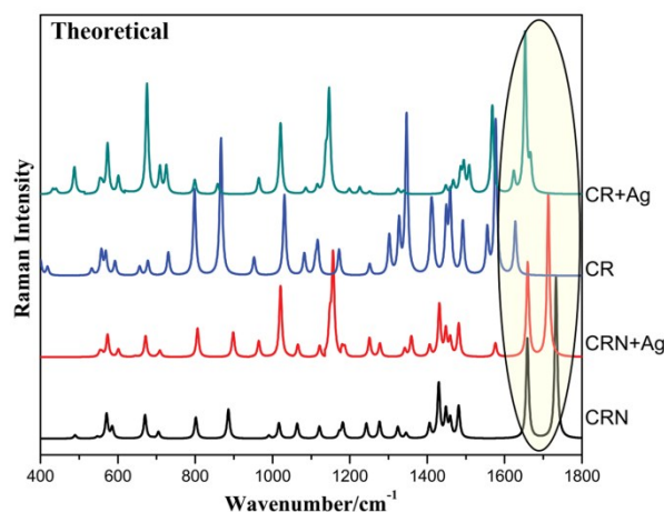
Fig. S1: Comparison between the DFT calculated Raman spectra of CRN and CR in aqueous solution and adsorbed on Ag surface. The spectra of CRN and CR show several changes when adsorbed on Ag surface, which show similar trend as observed in the SERS spectra.
